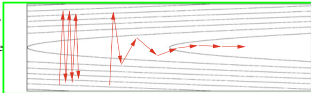
Fig. 9.24 Abrupt direction changes are smoothed out by the use of the momentum term. An iteration without the momentum term ( left ) in comparison to iteration with the momentum term ( right )
