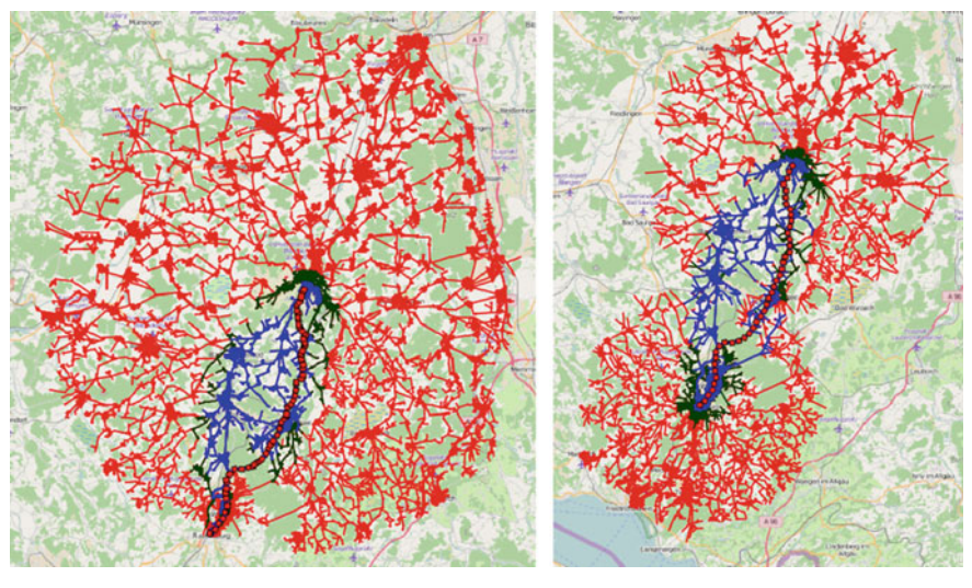
Fig. 6.18 A^* search tree without heuristic (red), with straight-line distance (dark green) and with landmarks (blue). The left image shows unidirectional search and the right shows bidirectional search. Note that the green edges are covered by blue and the red edges are covered by green and blue
