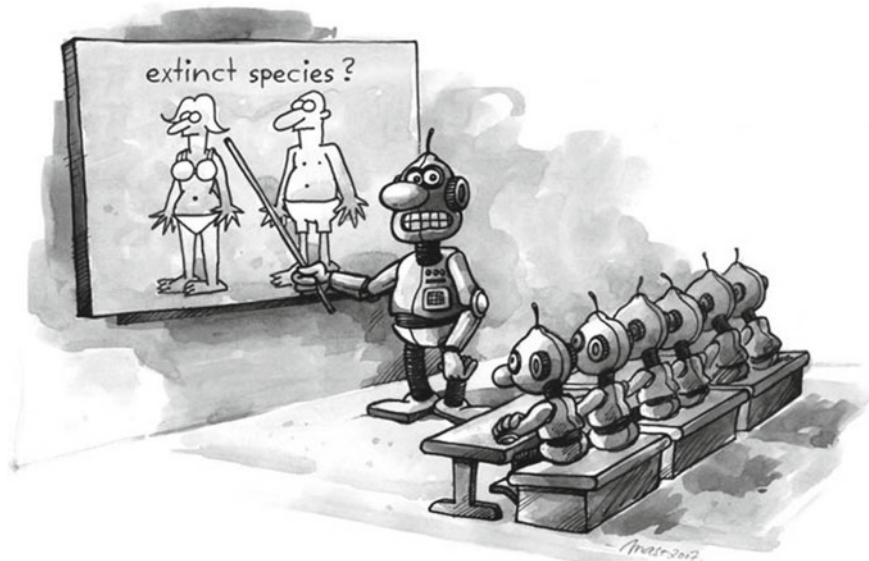
Fig. 8.1 Supervised learning ...
