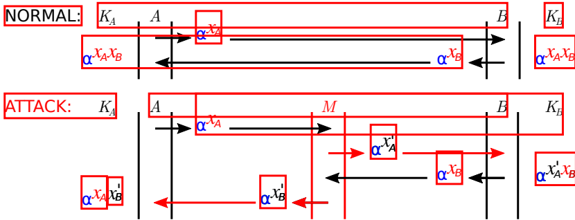
Fig. 5.14 A man-in-the-middle attack on the Diffie-Hellman protocol from an active attacker
