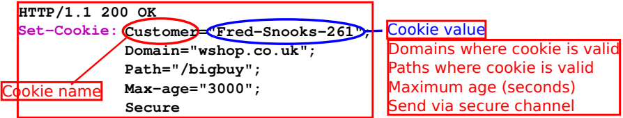
Fig. 10.14 A cookie transmitted in an HTTP response from a server to a client
