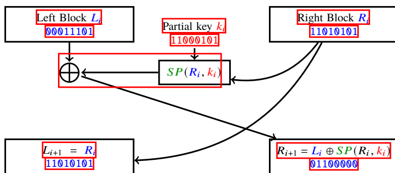
Fig. 4.7 Operation of a stage in a Feistel network
