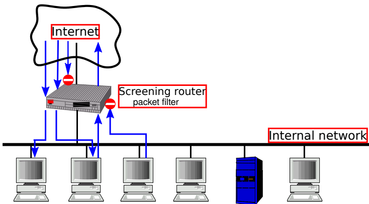
Fig. 8.20 A screening router setup
