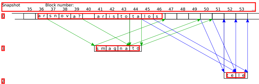
Fig. 11.6 Progress of work in a file system with snapshots
