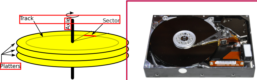
Fig. A.3 A classical HDD. Left: Schematic structure. Right: A physical disk with 3 platters.
