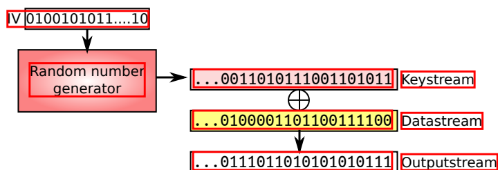
Fig. 4.13 Operation of a stream cipher.
