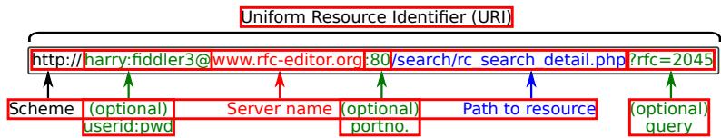
Fig. 7.10 The structure of a URI
