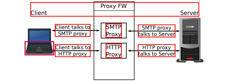
Fig. 8.19 An application proxy firewall
