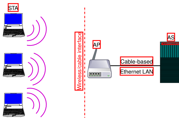
Fig. 8.25 Authentication with the use of 802.1X
