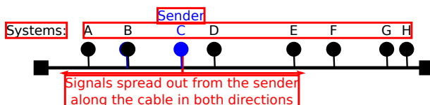
Fig. 6.15 Communication in Ethernet
