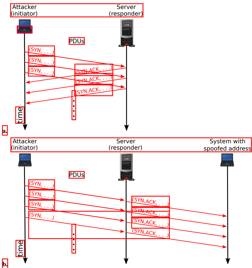
Fig. 8.30 DoS attacks in the Transport Layer
