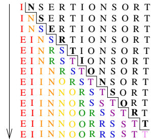
Figure 1.1: Animation of insertion sort in action (time flows downward).
