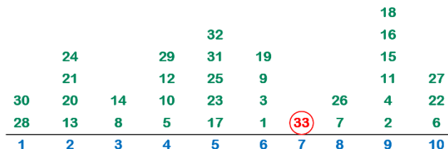
Figure 6.5: Illustrating the coupon collectors problem through an experiment tossing balls at random into ten bins. It is not until the 33rd toss that all bins are non-empty.
