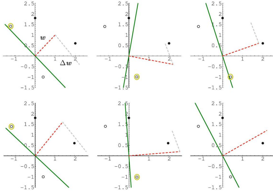
Figure 9.10: Application of the perceptron learning rule to two positive ( \cdot ) and two negative ( \circ ) data points. The solid line shows the current dividing line w \cdot x = 0 . The orthogonal dashed line is the weight vector w and the second dashed line the change vector \Delta w = x or \Delta w = -x to be added, which is calculated from the currently active data point surrounded in light green
