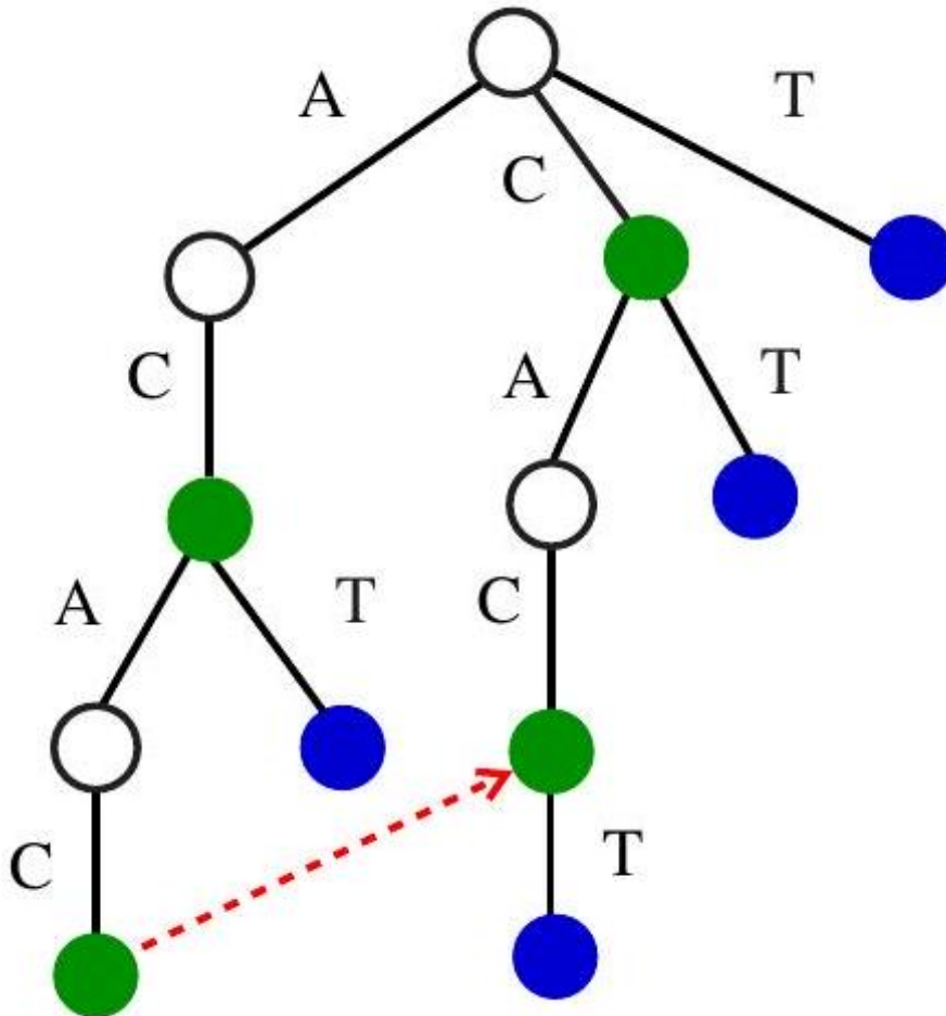
Figure 7.11: Suffix tree on ACAC and CACT , with the pointer to the suffix of ACAC . Green nodes correspond to suffixes of ACAC , with blue nodes to suffixes of CACT .
