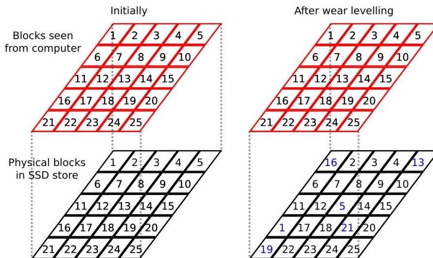
Fig. A. 4 Wear levelling in an SSD
