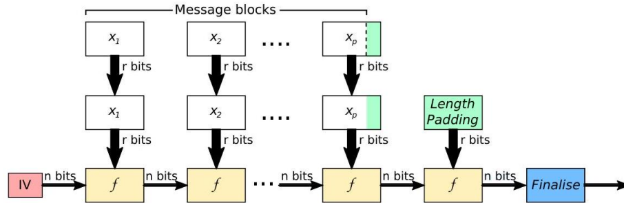
Fig. 8.2: Principle of operation of a cryptographic hash function based on the Merkle-Damgaard construction
