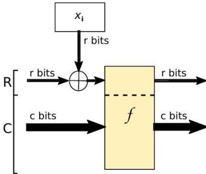
Fig. 8.3: r bits) and C (the capacity: c bits). Both R and C are initialised to 0. In each step, an input block is mixed with the R part of the current state using an XOR function, and then the function f is applied to both parts of the state to produce a random permutation of the (r + c) bits in the state. After the last block of input has been dealt with, the actual n -bit hash value is derived from the r bits in the R part of the final state.
