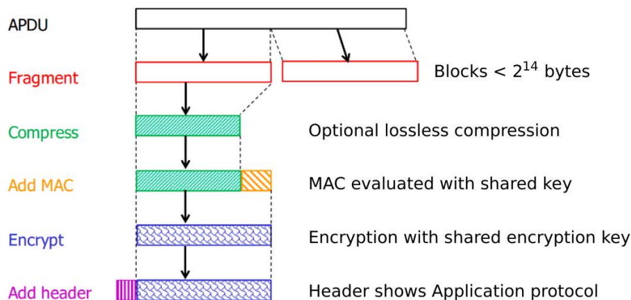
Fig. 11.12: Treatment of APDUs in SSL/TLS's Record protocol
