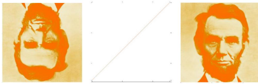
Figure 9.6: Multiplying the Lincoln matrix M by the reverse permutation matrix r (center). The product r \cdot M flips Lincoln upside down (left), while M \cdot r parts his hair on the other side of his head (right).
