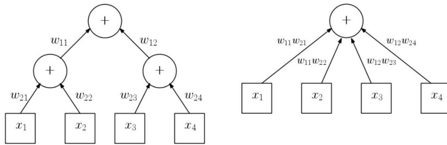
Figure 11.13: Addition networks do not benefit from depth. The two layer network (left) computes exactly the function as the equivalent one layer network (right).
