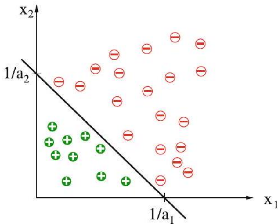
Figure 9.7: A linearly separable two dimensional data set. The equation for the dividing straight line is a_1x_1 + a_2x_2 = 1
