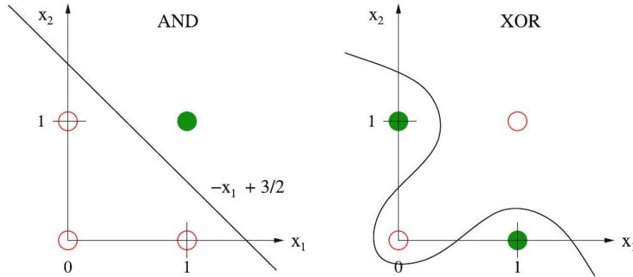
Figure 9.8: The boolean function AND is linearly separable, but XOR is not ( 0 \doteq \text{true} , 0 \doteq \text{false} )
