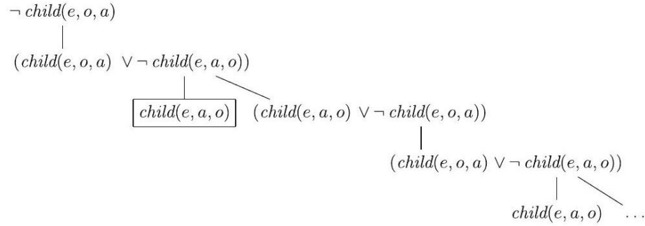
Figure 6.1: PROLOG search tree for child(eve, oscar, anne)
