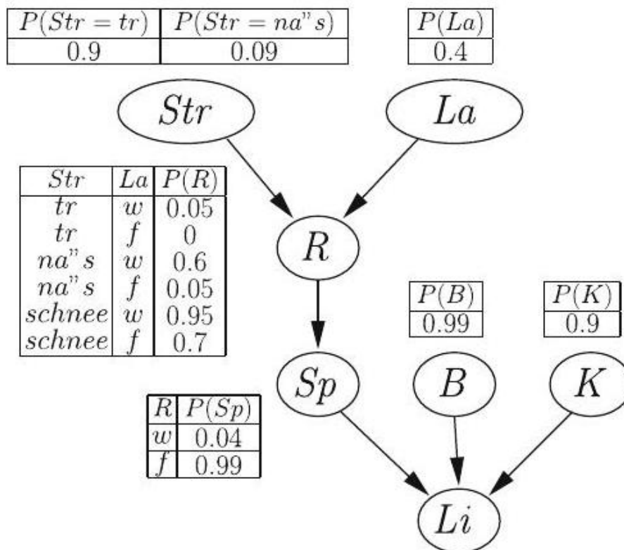
Figure 12.1: Bayesian network for the bicycle light. The CPT for Li is given in the problem statement
