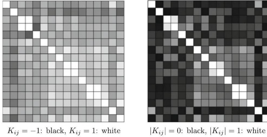
Figure 9.6: The correlation matrix as a frequency graph. In the left diagram, dark stands for negative and light for positive. In the right image the absolute values were listed. Here black means K_{ij} \approx 0 (uncorrelated) and white |K_{ij}| \approx 1 (strongly correlated)
