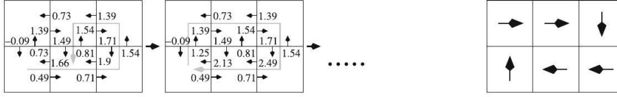
Figure 11.9: Q-learning applied to the example with n_x = 3, n_y = 2 . The gray arrows mark the actions carried out in each picture. The updated Q values are given. In the last picture, the current policy, which is also optimal, is shown
