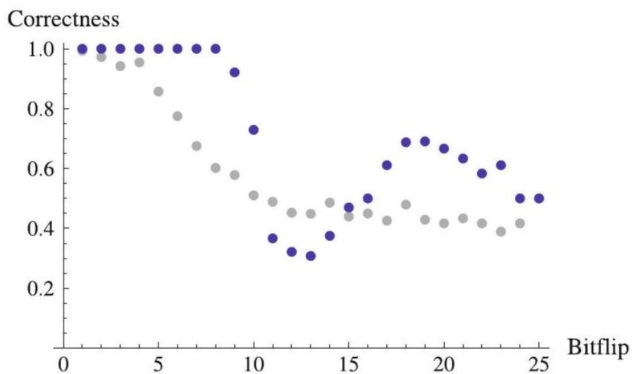
Figure 9.16: Relative correctness of nearest neighbor classification as a function of the number of inverted bits. The structure of the curve with its minimum at 13 and its maximum at 19 is related to the special structure of the training data. For comparison the values of the perceptron from Example 8.3 on page 188 are shown in gray
