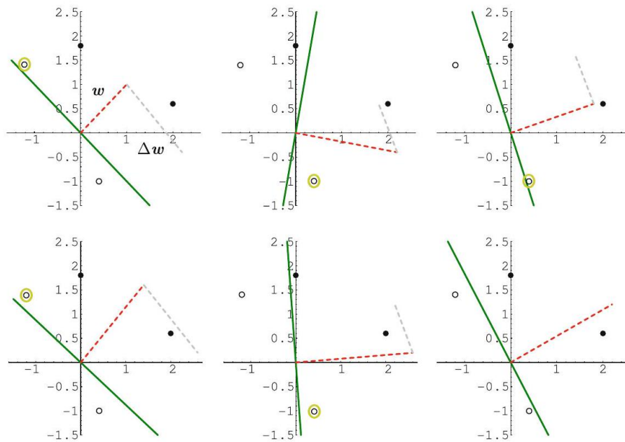
Figure 9.10: Application of the perceptron learning rule to two positive ( \bullet ) and two negative ( \circ ) data points. The solid line shows the current dividing line wx = 0 . The orthogonal dashed line is the weight vector w and the second dashed line the change vector \Delta w = x or \Delta w = -x to be added, which is calculated from the currently active data point surrounded in light green
