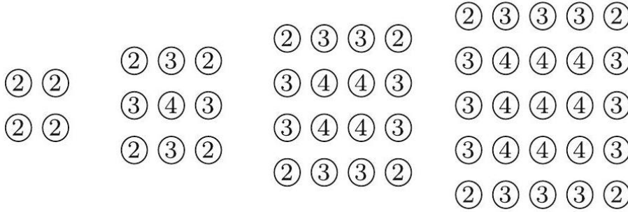
Figure 11.4: The state space for the example with the values 2, 3, 4, 5 for n_x and n_y . The number of possible actions is given for each state in the respective circles
