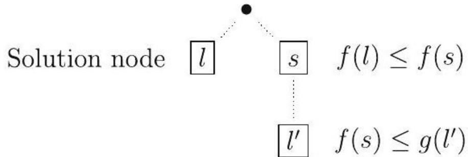
Figure 7.12: The first solution node l found by A^* never has a higher cost than another arbitrary node l'
