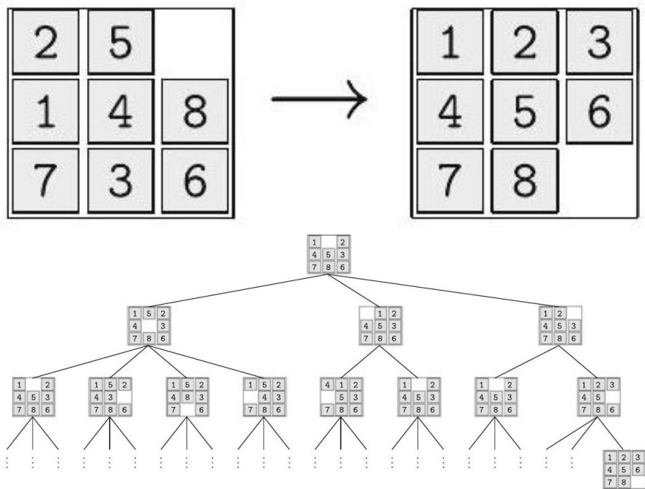
Figure 7.2: Possible starting and goal states of the 8-puzzle
