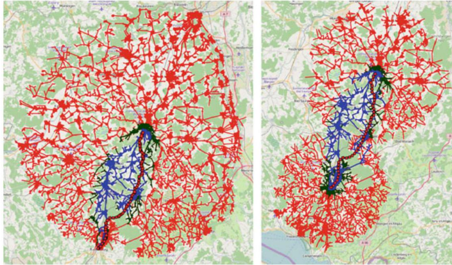
Fig. 6.18 A* search tree without heuristic (red), with straight-line distance (dark green) and with landmarks (blue). The left image shows unidirectional search and the right shows bidirectional search. Note that the green edges are covered by blue and the red edges are covered by green and blue
