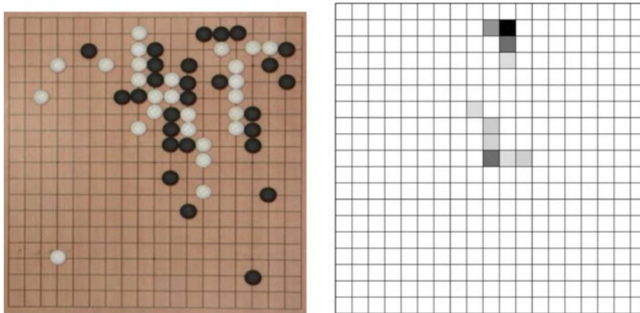
Figure 11.10: Density graph (right) of a move probability p_{\sigma}(a | s) for the player with white stones in the board state shown on the left. For each white square, p_{\sigma}(a | s) = 0 . The darker the square, the higher the value for a move by white onto the corresponding grid point
