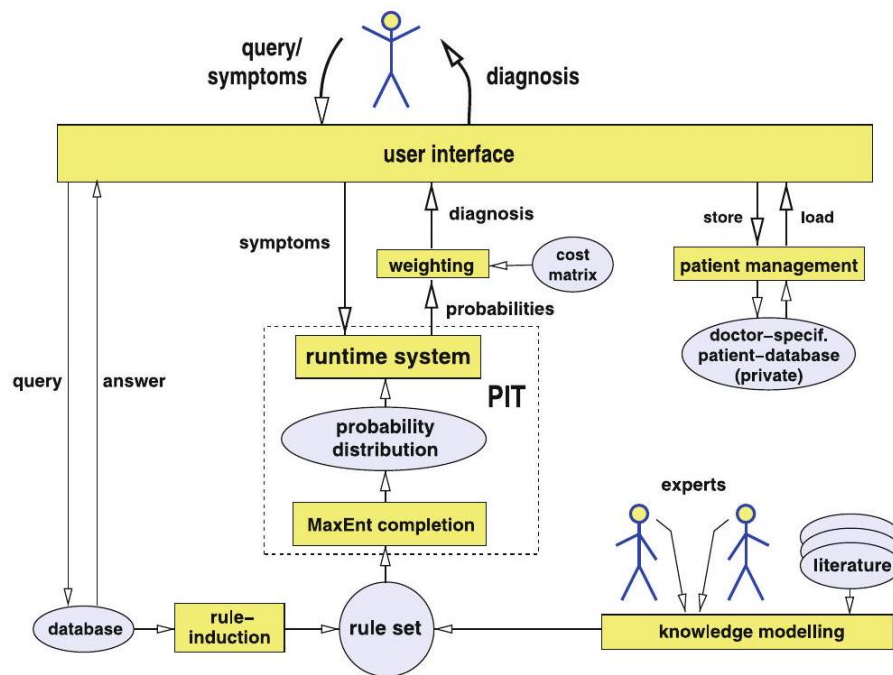
Figure 8.5: Rules are generated from the database as well as from expert knowledge. From these, MaxEnt creates a complete probability distribution. For a user query, the probability of every possible diagnosis is calculated. Using the cost matrix (see Sect. 7.3.5) a decision is then suggested
