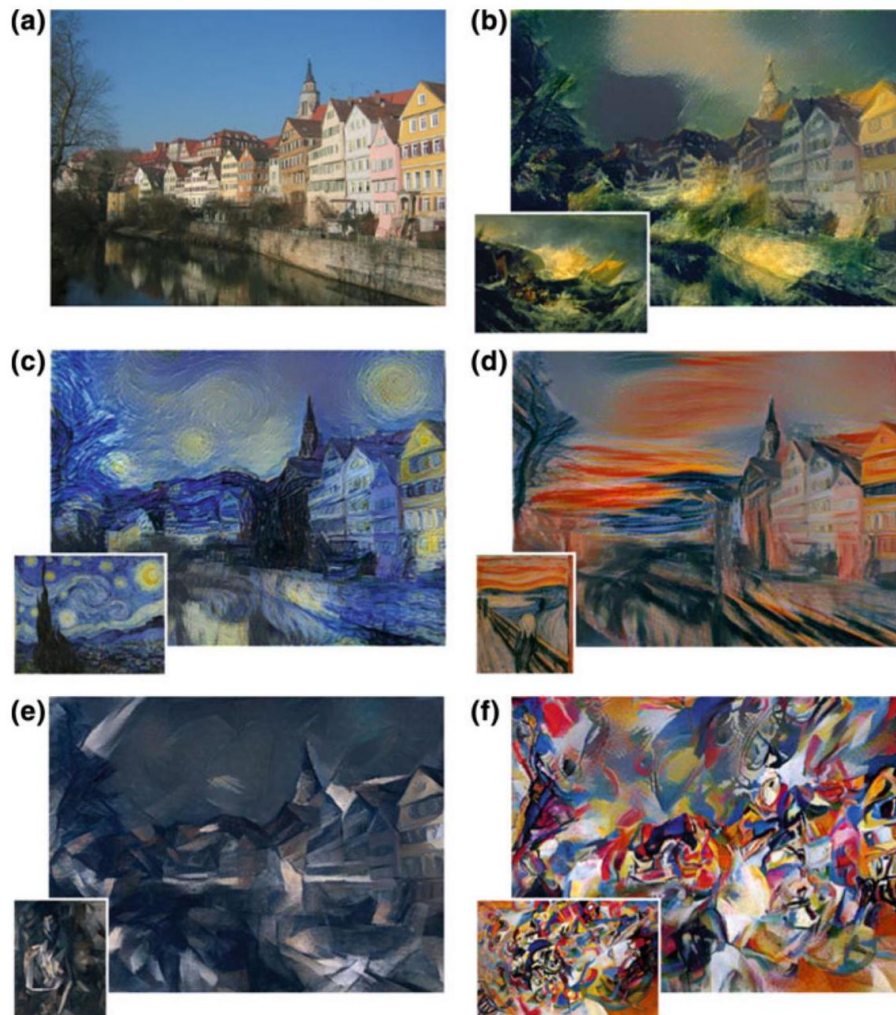
Figure 10.23: Artistic pictures of the view of Tübingen in the top left generated with the network from [citegatys2015neural]. For each pair of images, the famous painting whose style was used to transform the photo can be seen in the bottom left (Source [citegatys2015neural])
