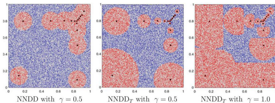
Figure 9.29: NNDD and NNDD T applied to a set of 16 selected two-dimensional data points (black points). In each case, class membership has been determined for 10,000 randomly selected points. The points marked in red were classified as positive, i.e. assigned the training set's class, while the blue points are classified as negative
