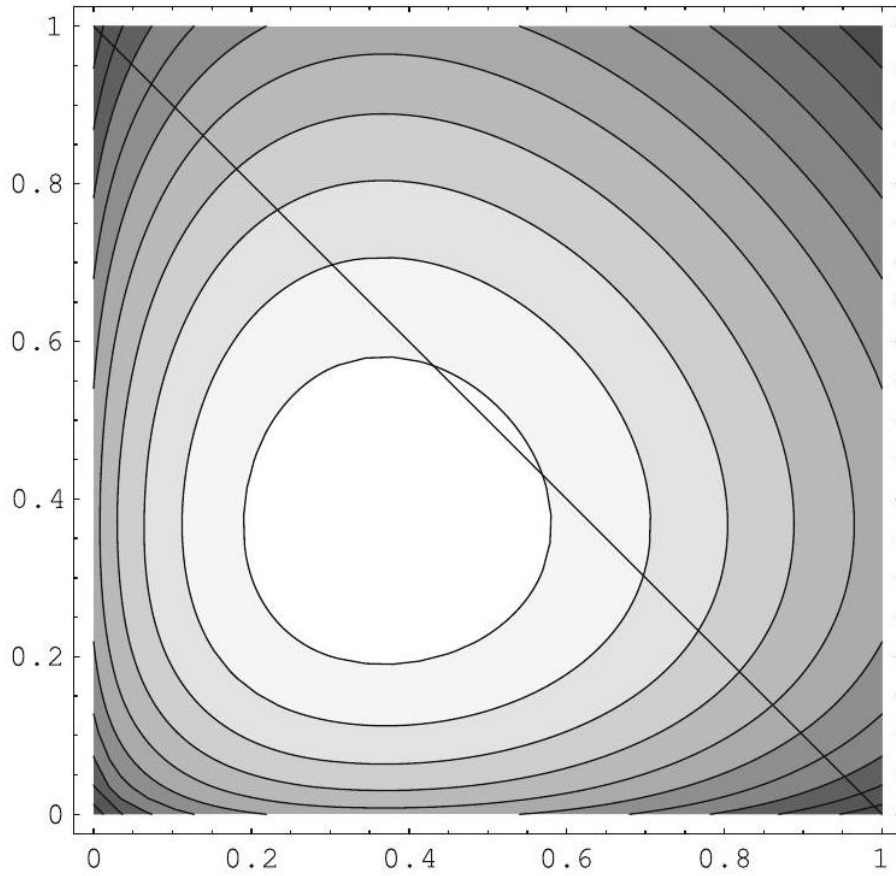
Figure 8.2: Contour line diagram of the two-dimensional entropy function. We see that it is strictly convex in the whole unit square and that it has an isolated global maximum. Also marked is the constraint p_3 + p_4 = 1 as a special case of the condition p_3 + p_4 - 1 + \alpha = 0 for \alpha = 0 which is relevant here
