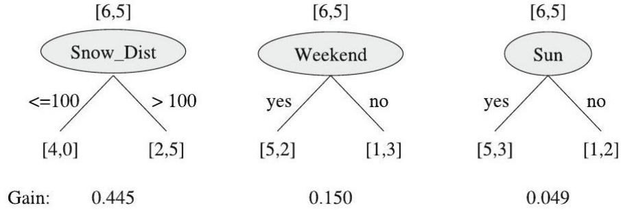
Figure 9.23: The calculated gain for the various attributes reflects whether the division of the data by the respective attribute results in a better class division. The more the distributions generated by the attribute deviate from the uniform distribution, the higher the information gain
