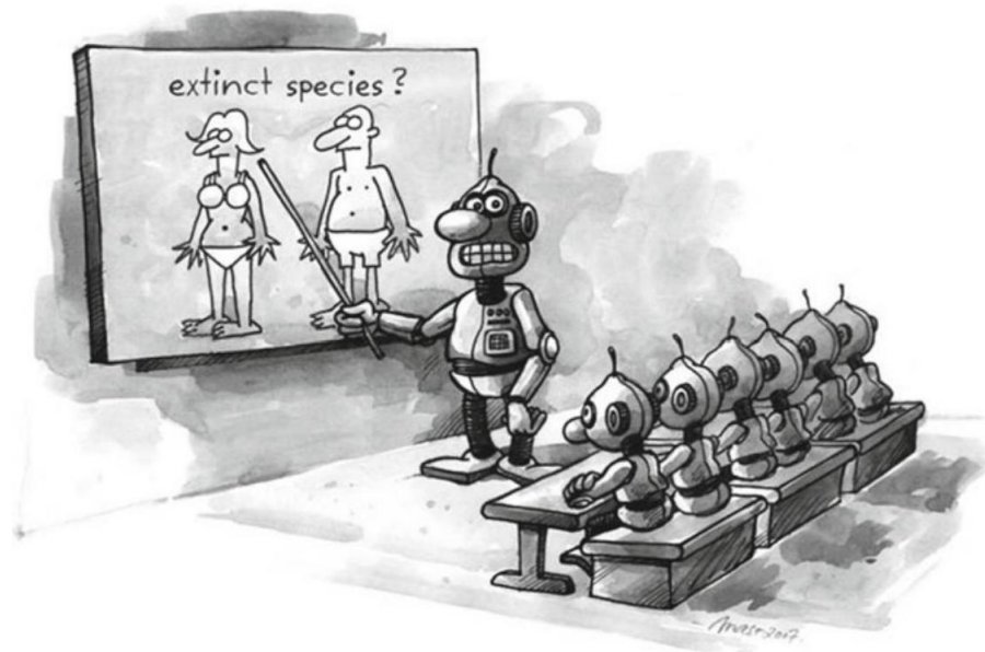
Figure 9.1: Supervised learning ...
