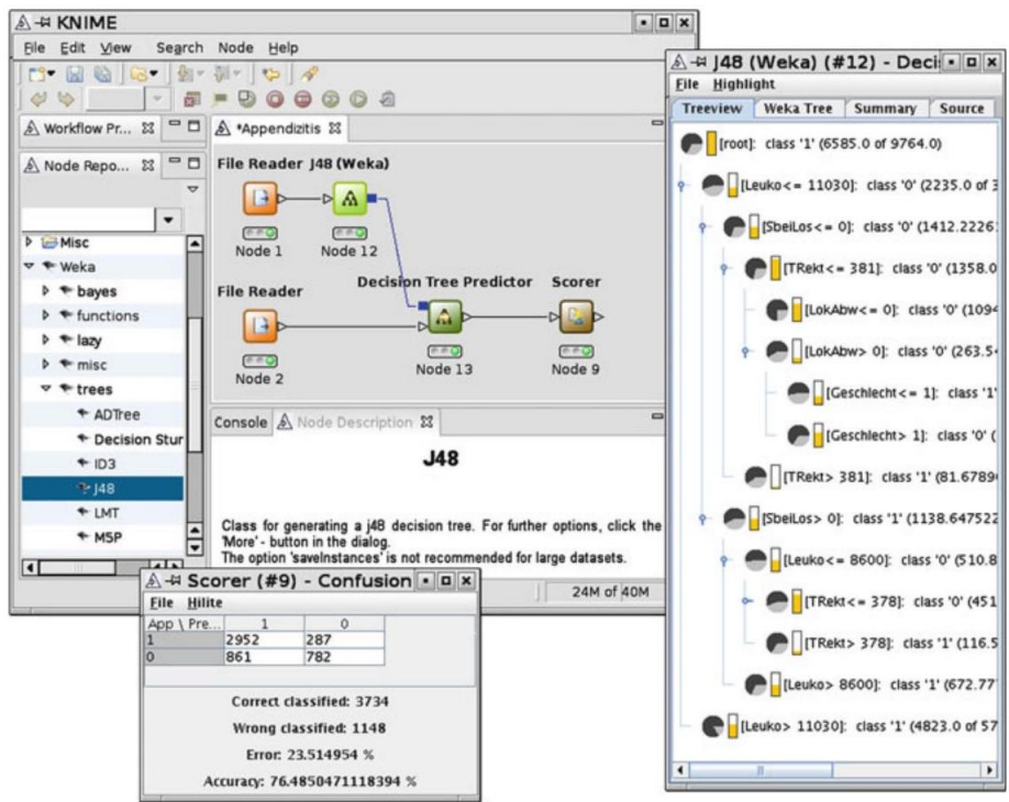
Figure 9.36: The KNIME user interface with two additional views, which show the decision tree and the confusion matrix
