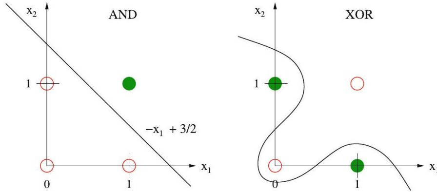
Figure 9.8: The boolean function AND is linearly separable, but XOR is not ( 0 \doteq \text{true} , 0 \doteq \text{false} )
