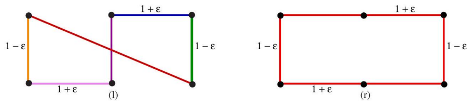
Figure 1.4: A bad instance for the closest-pair heuristic, with the optimal solution.
