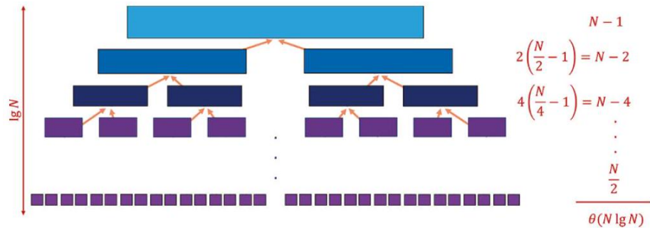
Figure 4.4: The recursion tree for mergesort. The tree has height \lceil \lg n \rceil , and the cost of the merging operations on each level are \Theta(n) , yielding an \Theta(n \lg n) time algorithm.
