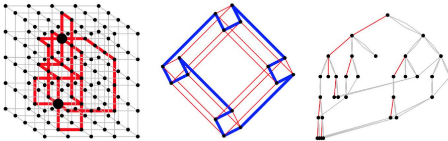
Figure 7.6: Representative Combinatorial graphs: edge-disjoint paths (left), Hamiltonian cycle in a hypercube (center), animated depth-first search tree traversal (right).
