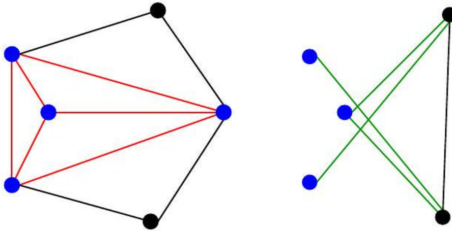
Figure 11.6: A small graph with a four-vertex clique (left), with the corresponding independent set in black forming a two-vertex clique in the graph's complement (right).
