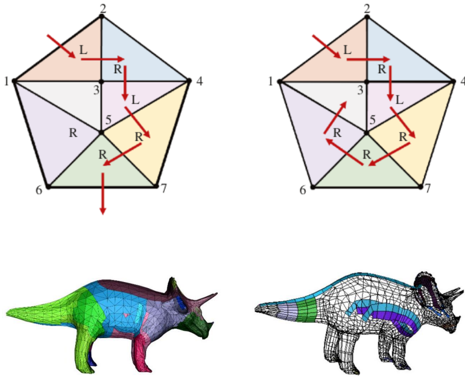
Figure 3.6: A triangulated model of a dinosaur (l), with several triangle strips peeled off the model (r).
