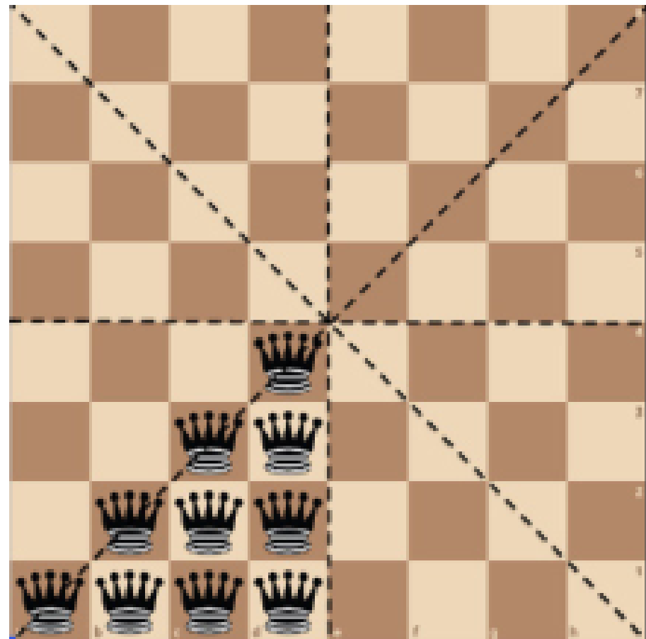
Figure 9.5: Configurations covering 63 but not 64 squares.
