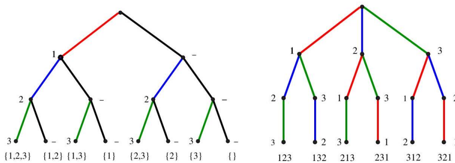
Figure 9.1: Search tree enumerating all subsets (left) and permutations (right) of {1, 2, 3}. The color of the search tree edges reflects the element being inserted into the partial solution.
