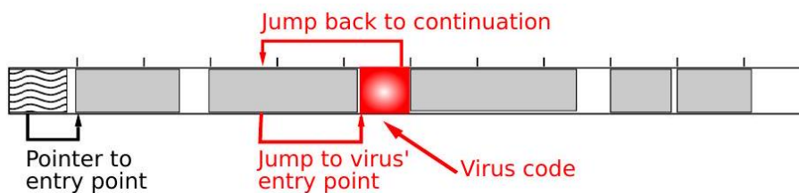
Fig. 13.4: Placement of virus code in an executable file.
