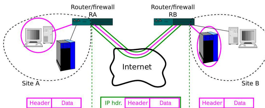
Fig. 11.8: Site-to-site tunneling
