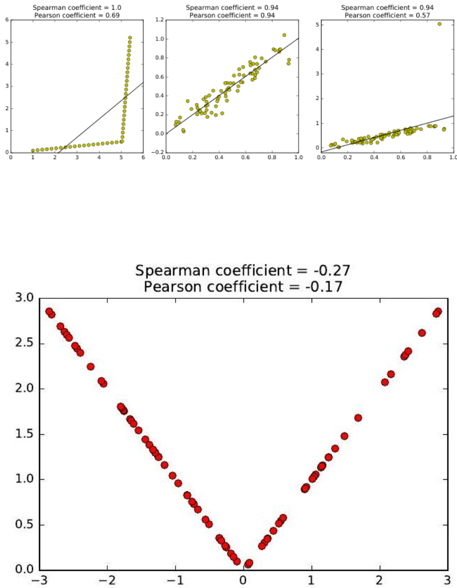
Figure 4.6: The function y = |x| does not have a linear model, but seems like it should be easily fitted despite weak correlations.
