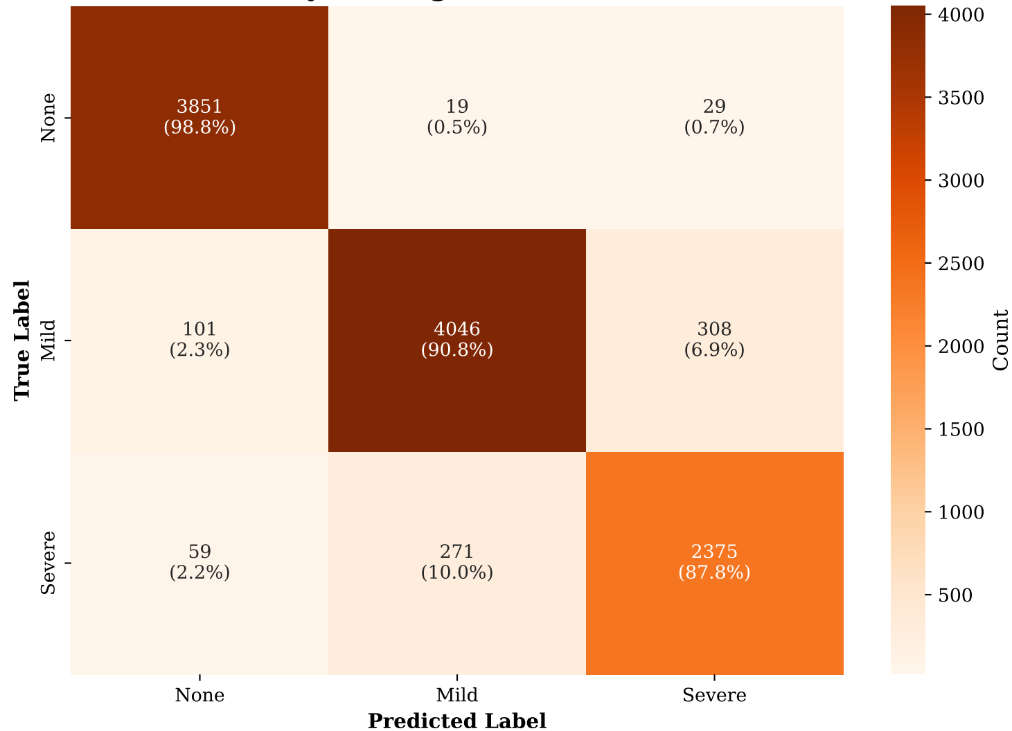
Severity Grading Confusion Matrix
