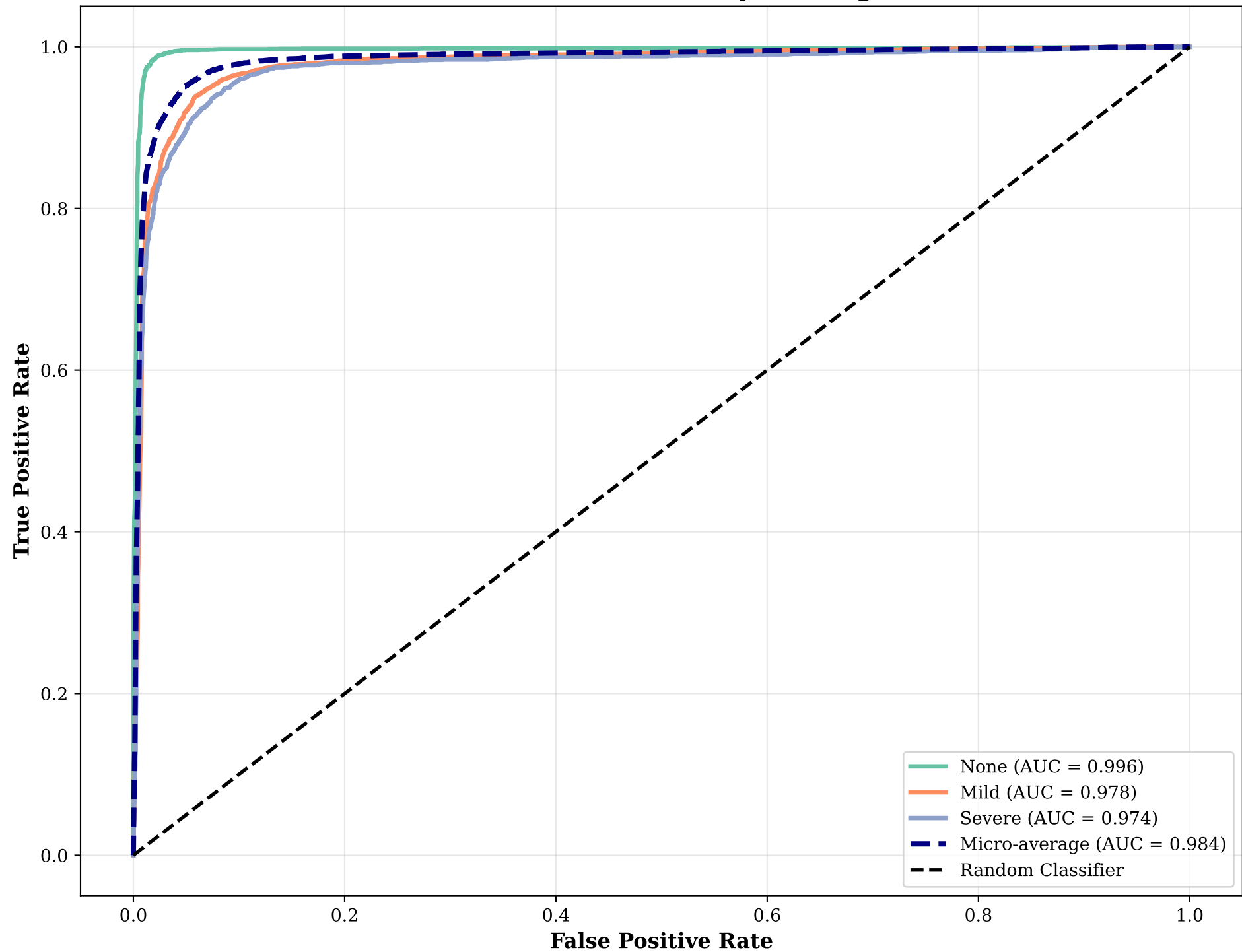
ROC Curves - Severity Grading
