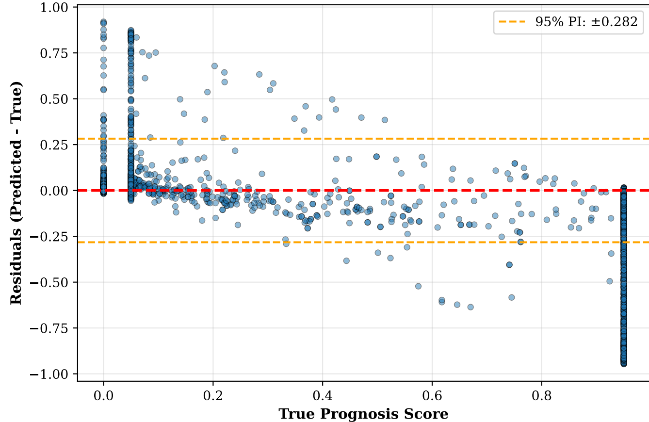
Residual Plot with Prediction Intervals
