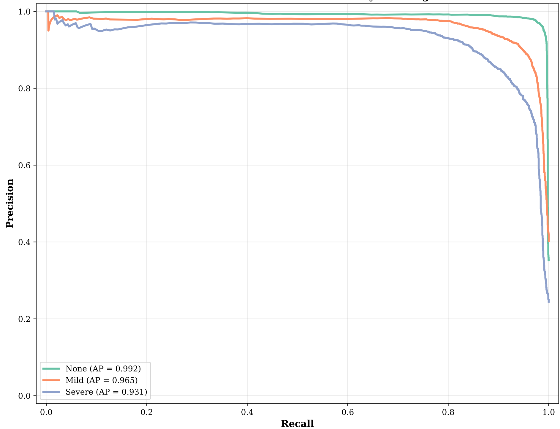
Precision-Recall Curves - Severity Grading
