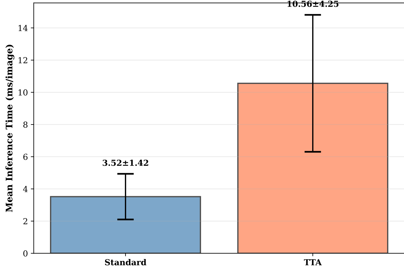
Mean Inference Time with Std Dev
