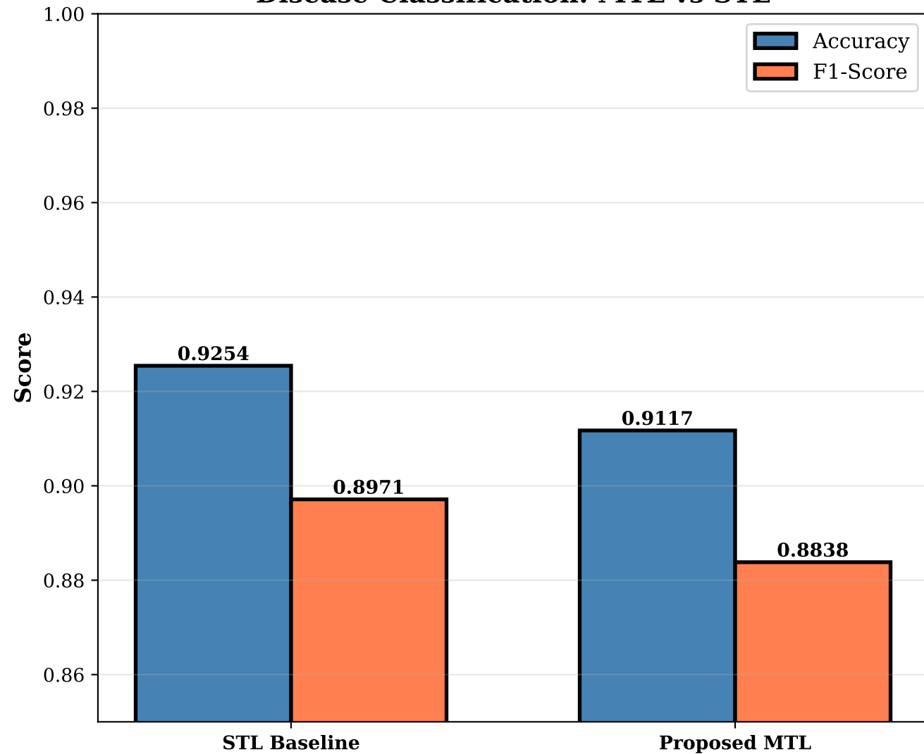
Disease Classification: MTL vs STL
