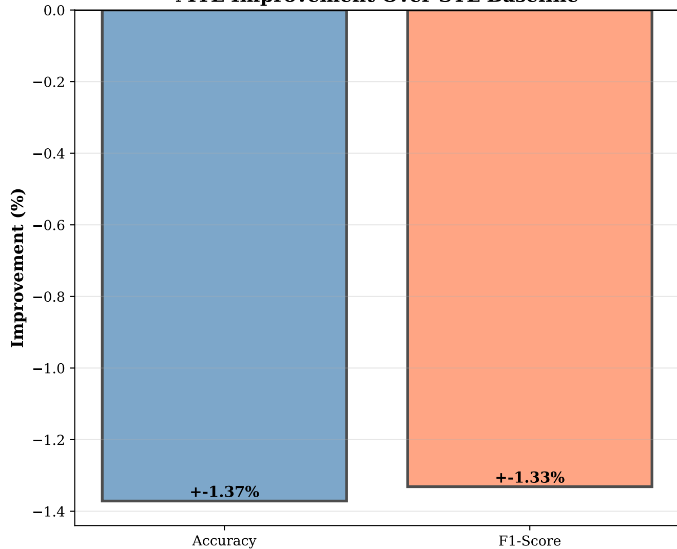
MTL Improvement Over STL Baseline
