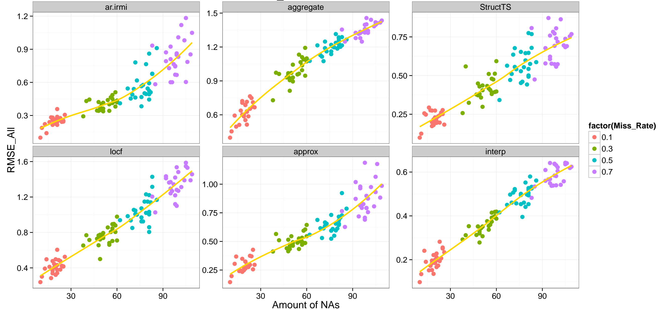
RMSE_All for beersales
