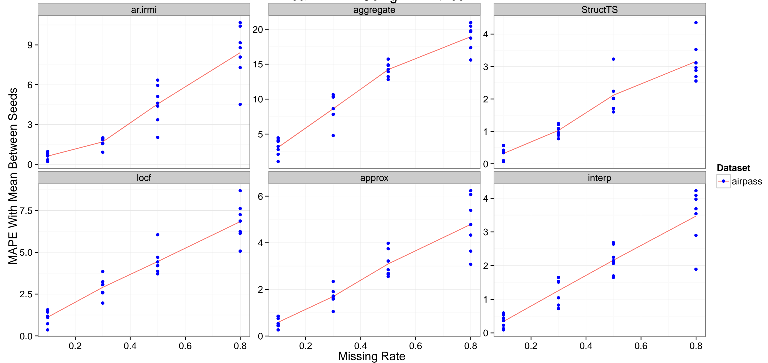
Mean MAPE Using All Entries
