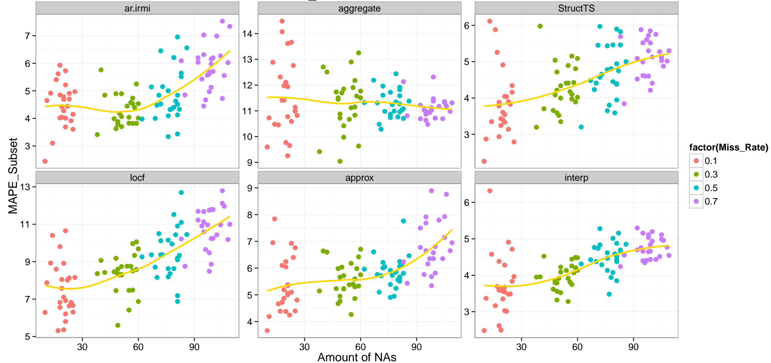
MAPE_Subset for beersales
