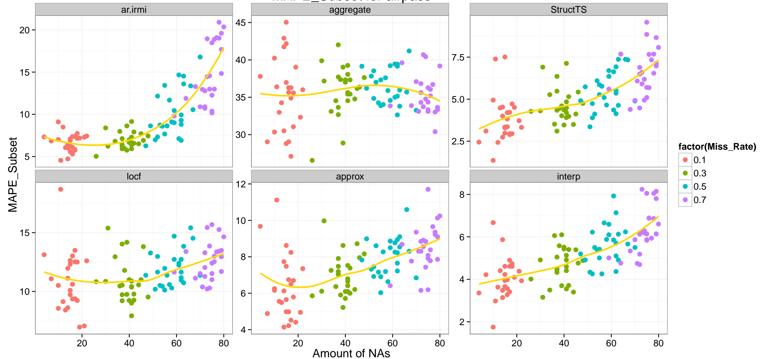
MAPE_Subset for airpass
