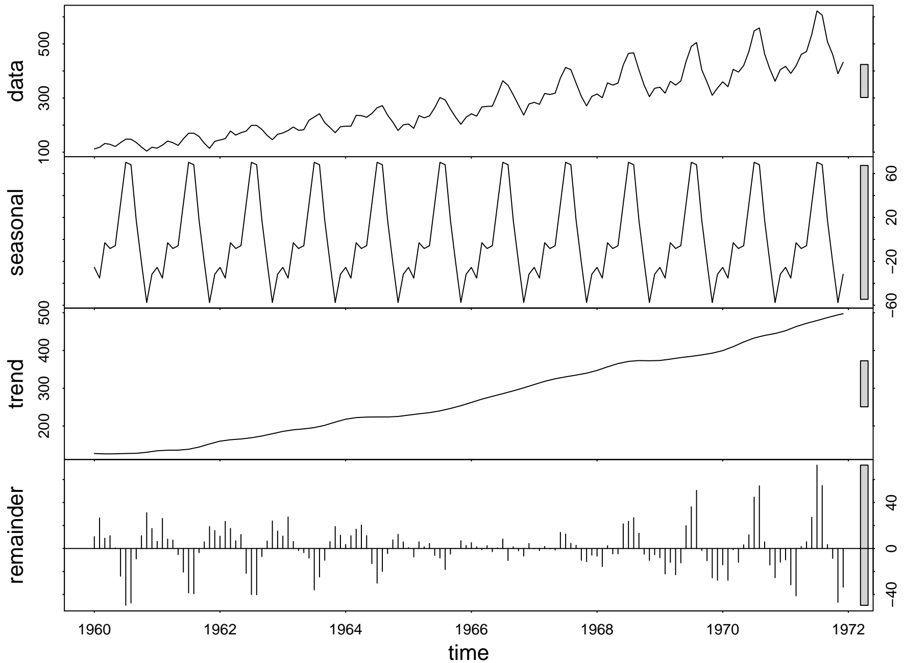
Loess Seasonal Decomposition of airpass
