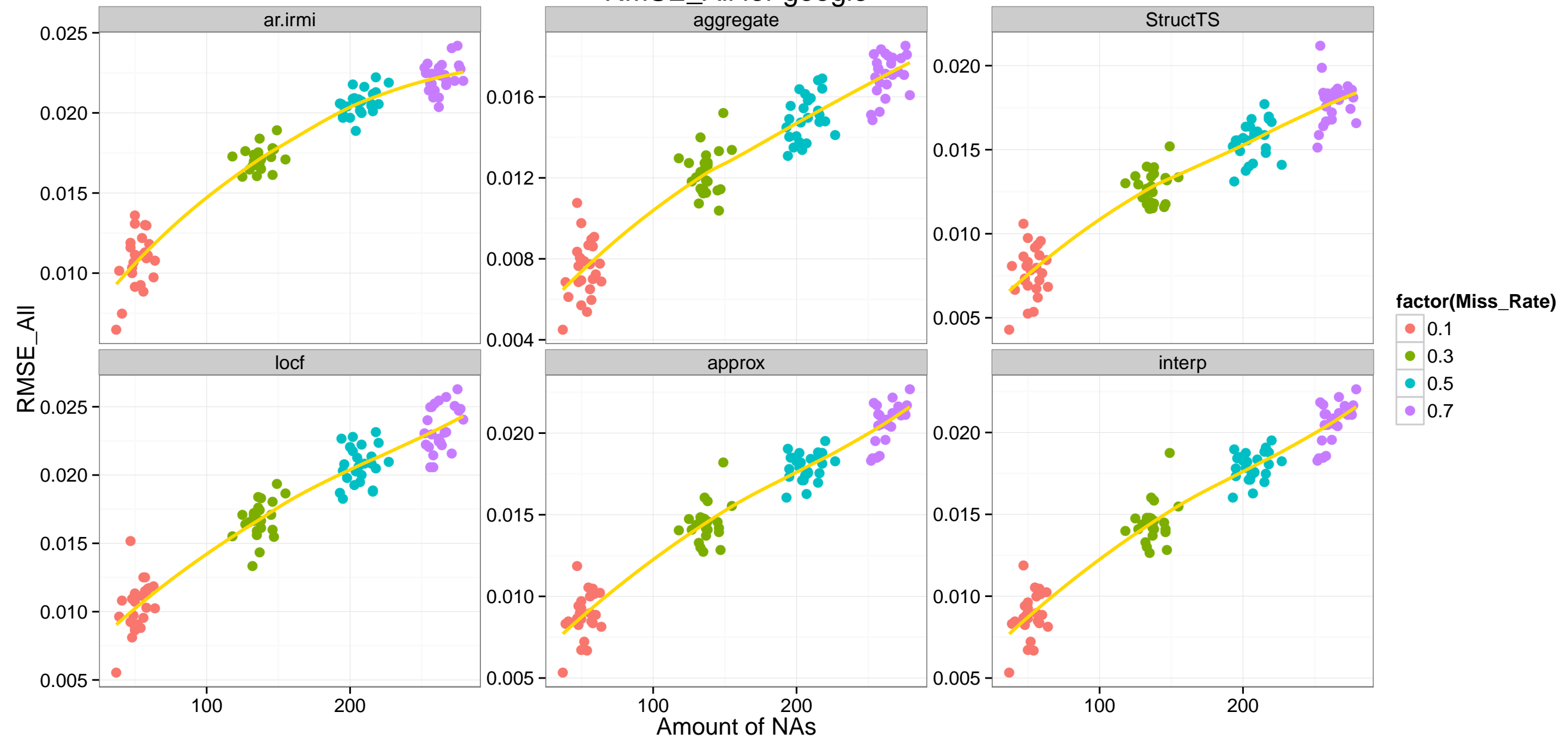
RMSE_All for google
