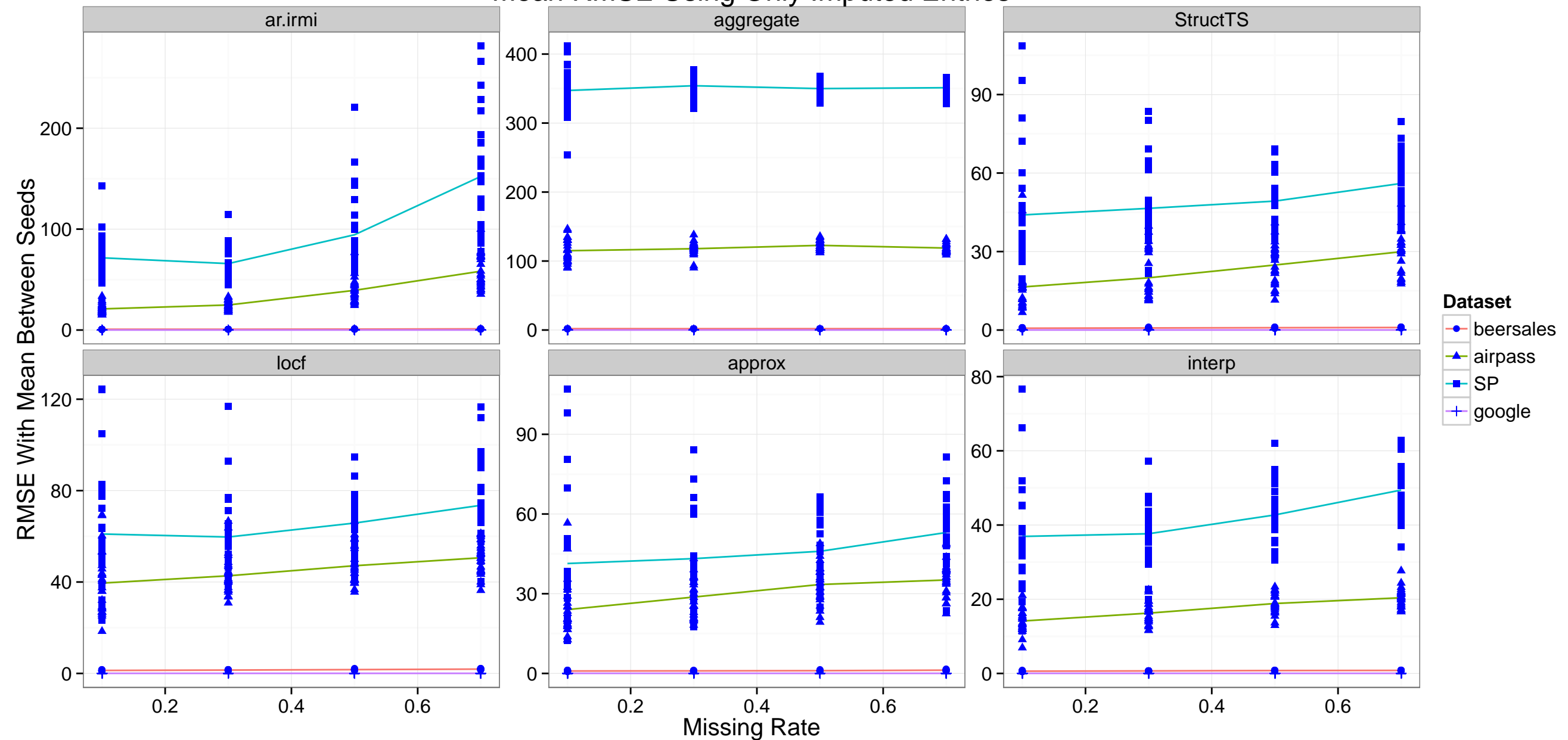
Mean RMSE Using Only Imputed Entries
