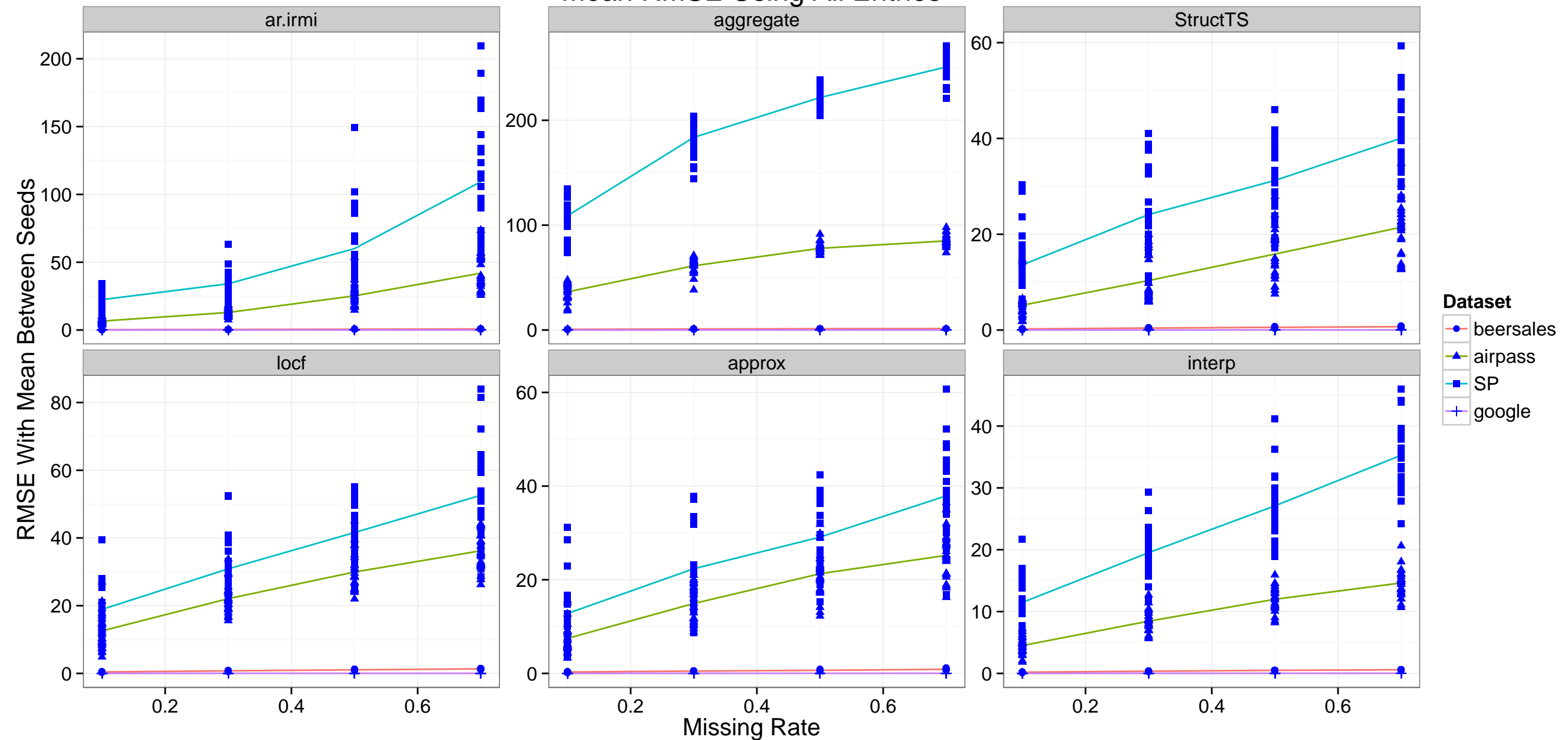
Mean RMSE Using All Entries
