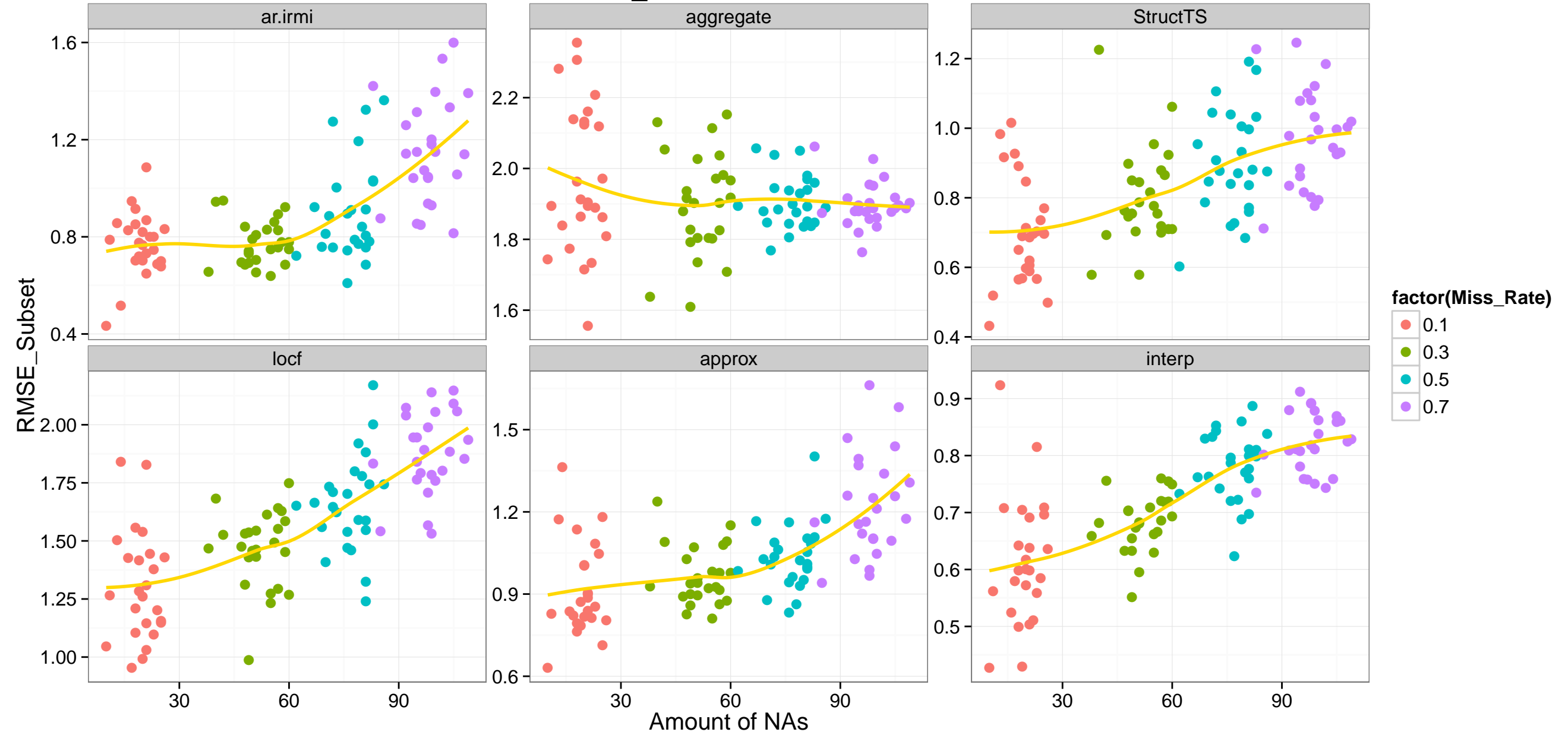
RMSE_Subset for beersales
