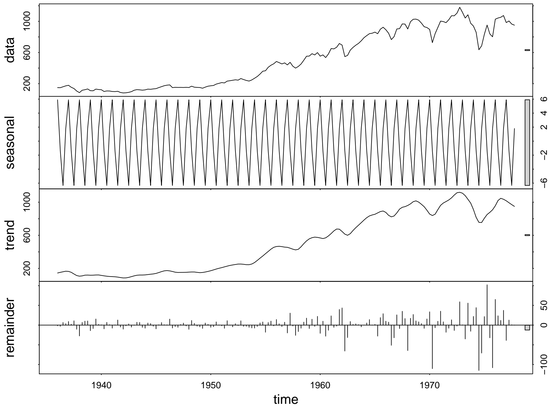
Loess Seasonal Decomposition of SP
