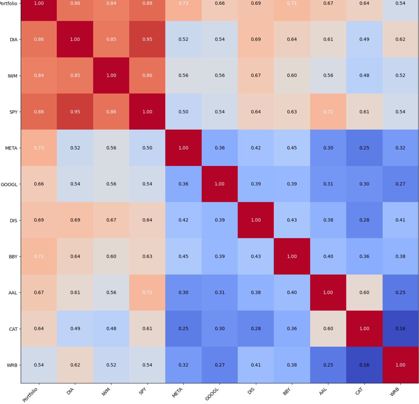
Correlation Matrix Heatmap
