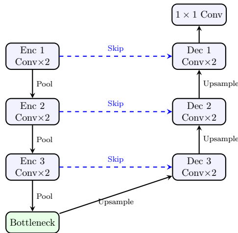
Figure 2.2: Standard U-Net encoder-decoder architecture with skip connections [1].
