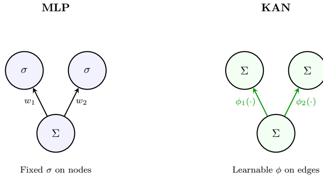
Figure 2.1: MLP vs KAN [9].
