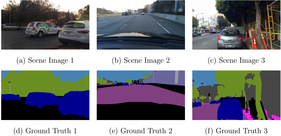
Figure 2.3: Sample 2 \times 3 grid from the BDD100K dataset: top row shows RGB driving scene images, bottom row shows the corresponding pixel-level ground truth semantic segmentation color labels [3].
