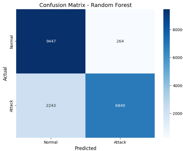
Figure 2: NSL-KDD: Confusion matrix visualization showing classification distribution, with emphasis on how well the models minimize false positives and false negatives.
