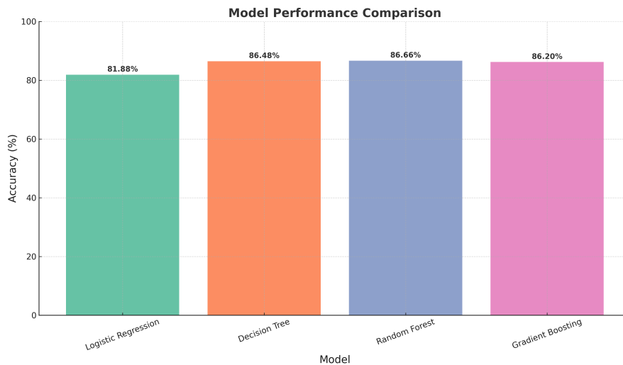
Figure 1: NSL-KDD: Model accuracy comparison showing that Random Forest slightly outperforms other models, while Logistic Regression performs lowest, highlighting the difference in handling nonlinear attack traffic.
