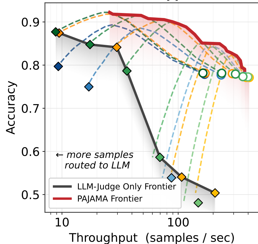
Oracle Router (Upper Bound)
