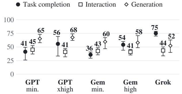
Fig. 1. Fixed-system means with worst-to-best language ranges. Task completion and Interaction average six languages; Generation averages the five localized languages.
