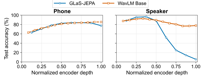
Fig. 4. Phone and speaker linear-probe test accuracy versus normalized encoder depth for GLaS-JEPA and WavLM Base.
