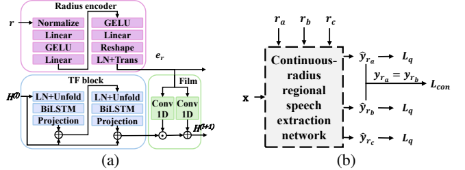
Fig. 3. (a) TF block with radius conditioning and (b) cross-radius consistency learning.
