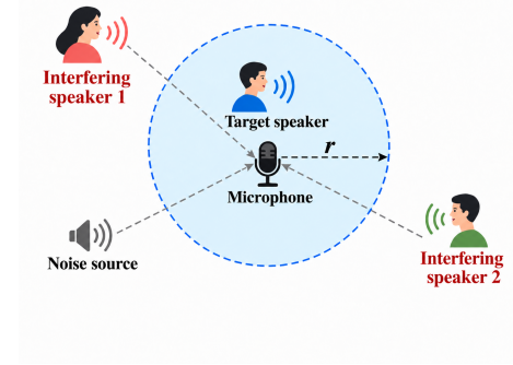
Fig. 1. Continuous-radius regional speech extraction task.
