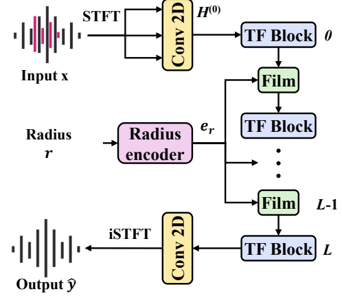
Fig. 2. Continuous-radius extraction network.
