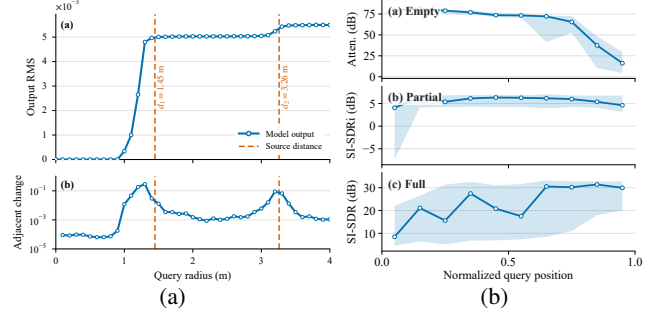
Fig. 4. Continuous-radius analysis: (a) response of a representative mixture and (b) aggregated dense-query performance.
