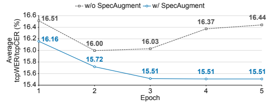
Figure 3: Average tcpWER/tcpCER of Qwen3-ASR-FT across training epochs, with and without SpecAugment.
