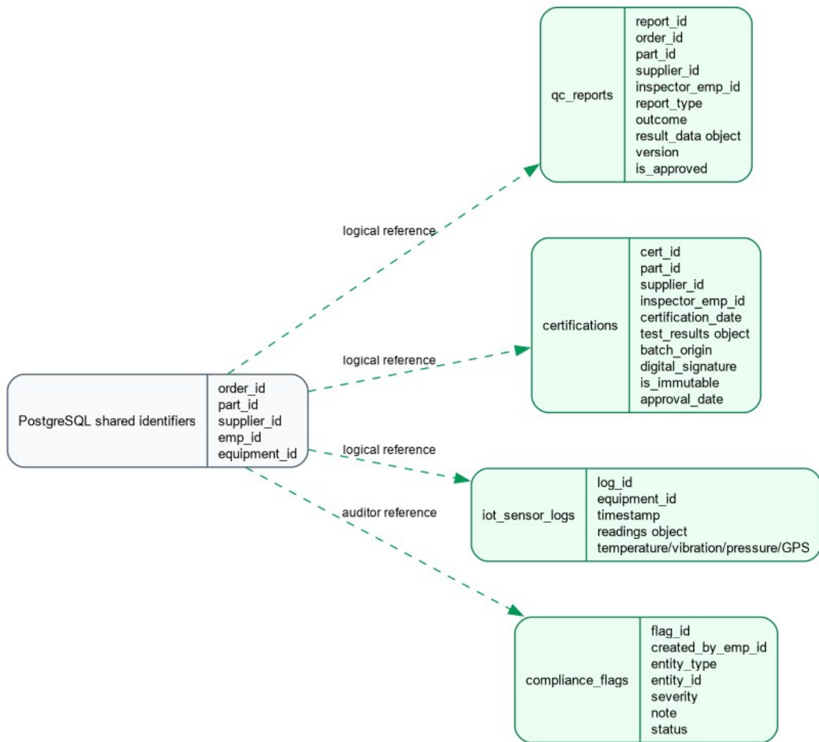
Figure 2 - Refined MongoDB document model
