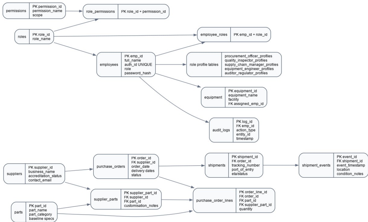
Figure 1 - Refined PostgreSQL relational schema
