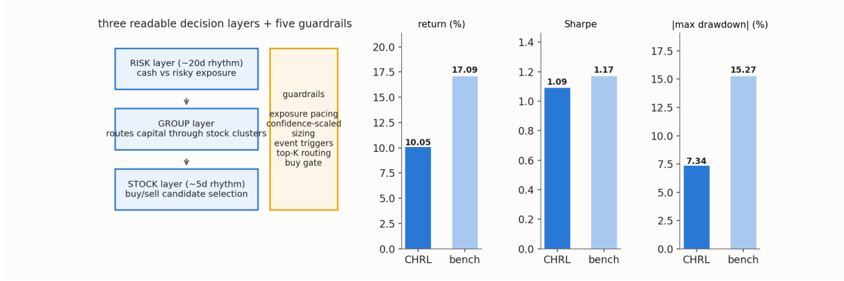
Figure 1: CHRL. Left: the three-layer decision factorization and its five guardrails — each stage emits a loggable, auditable signal on its own rhythm. Right: four-fold walk-forward validation against the 100%-risky equal-weight benchmark: 58.8% of the return, 93.2% of the Sharpe, 52% less drawdown.
