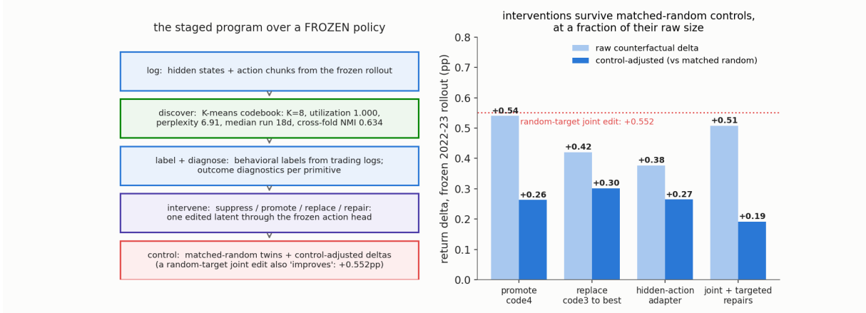
Figure 2: The Interpretable-CHRL program. Left: the staged pipeline over the frozen policy — log, discover ( K=8 codebook; utilization 1.000; perplexity 6.91; median run 18d; cross-fold NMI 0.634), label, diagnose, intervene (Eq. 2), control. Right: the flagship counterfactuals on the frozen 2022–23 rollout, raw vs control-adjusted; the dotted line is the random-target joint edit (+0.552 pp) that makes control adjustment mandatory.
