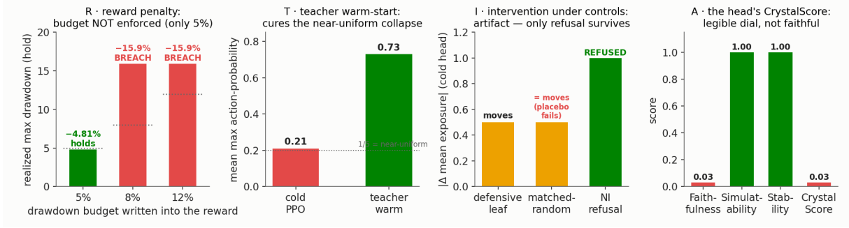
Figure 5: The four influence levers on the real daily panel, under controls. R: the reward penalty holds only the 5% budget — the penalty does not enforce the budget. T: the teacher warm-start cures the cold near-uniform collapse ( 0.21 \rightarrow 0.73 ; corrected contrast-write F = 0.77\text{--}0.83 ). I: a matched-random leaf moves the cold head as much as the targeted one — only the non-inferiority refusal (Eq. 14) survives. A: the cold head is a legible, stable dial ( S=1.0 , St=1.0 , F=0.03 ), not a faithful command surface.
