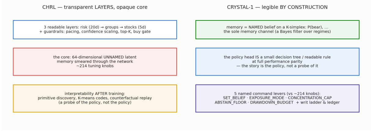
Figure 3: The journey in one picture. CHRL factors decisions into readable layers but keeps an unnamed 64-d latent core with \sim 214 knobs, explained only after training (§3). CRYSTAL-1 makes the explanation the mechanism: a named belief as the sole memory channel, a readable rule as the policy itself, and five named command levers.
