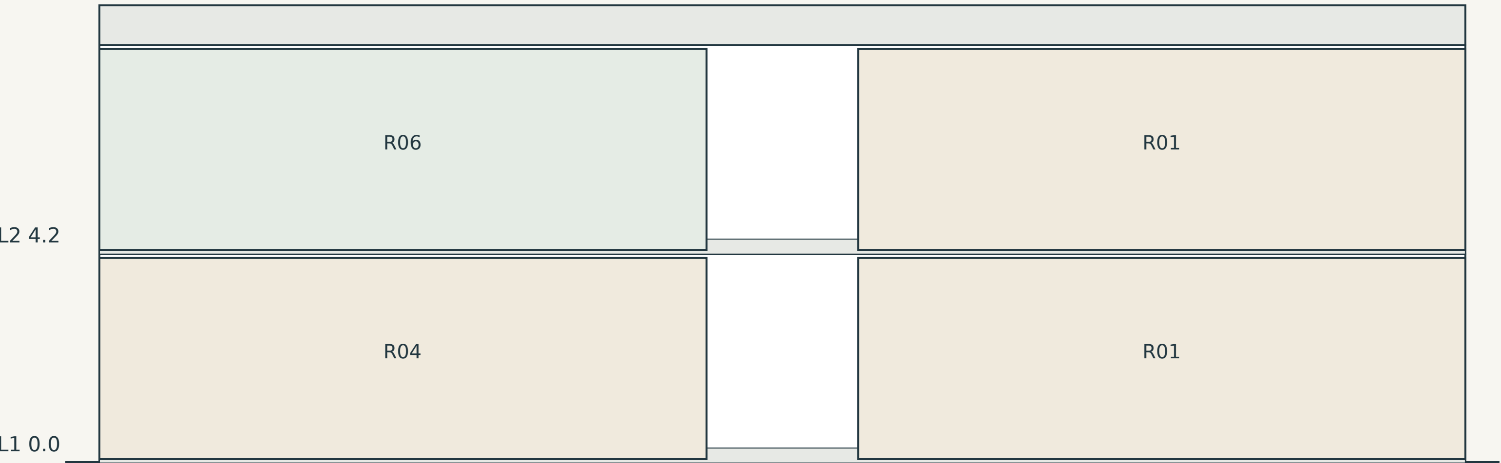
Span 27.43 m • top of modelled stack 8.40 m Cut offset 15.36 m from west edge. Tags: floor schedules; dashed: program zones.
