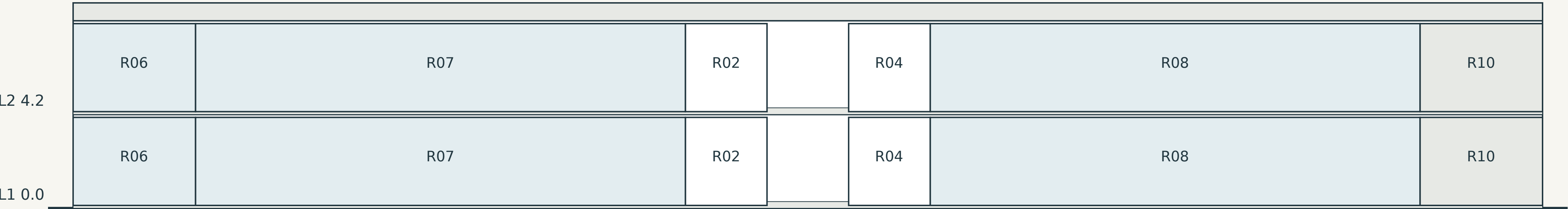
Span 65.84 m • top of modelled stack 8.40 m Cut offset 23.77 m from south edge. Tags: floor schedules; dashed: program zones.
