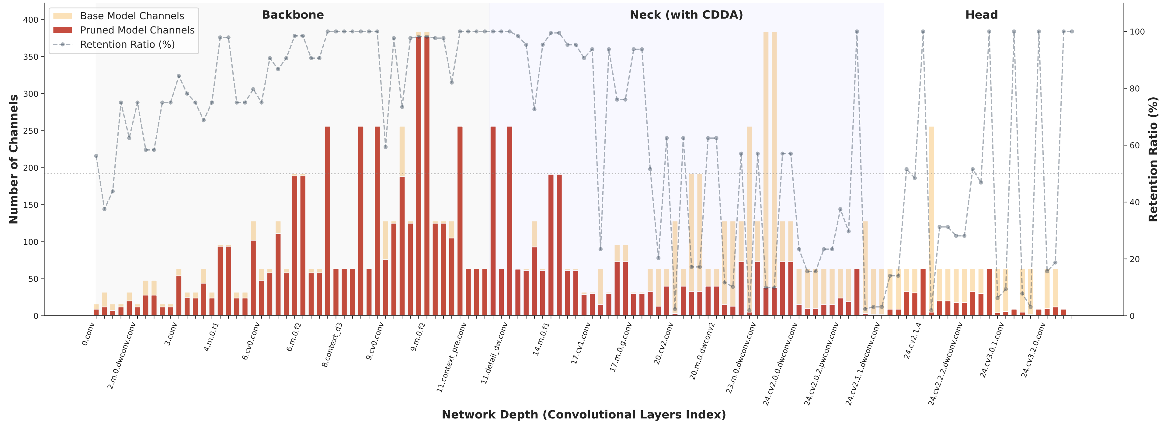
SLC-YOLOv8n: Structural Compression and Channel Retention Analysis
