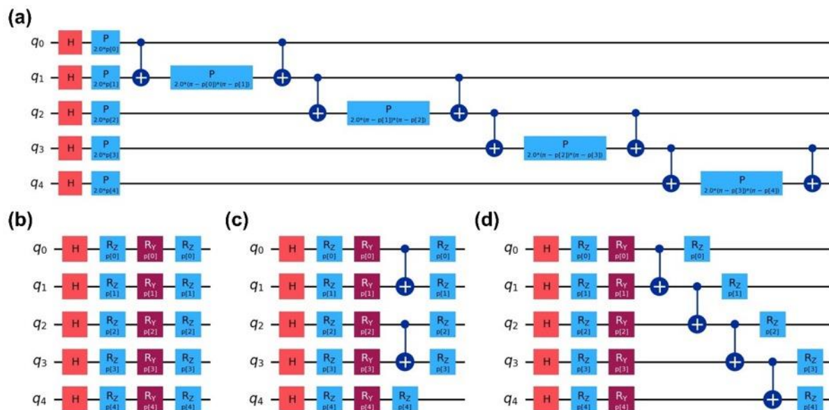
Different Quantum Circuit Architectures and Entanglement Levels
