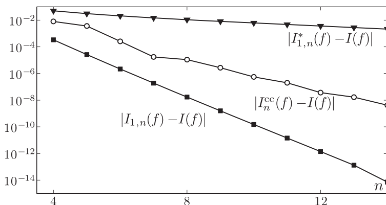
Figure 4.8 Semi-logarithmic plot of the absolute quadrature errors corresponding to the three methods used to approximate I(f) = 10 \int_0^\pi (1 - (9/25)\cos^2\theta)^{1/2} d\theta . From bottom to top: Composite trapezoidal (black squares), Clenshaw–Curtis (hollow circles), and composite trapezoidal applied with previous splitting of the domain of integration [0, \pi/4] and [\pi/4, \pi] (black triangles).
