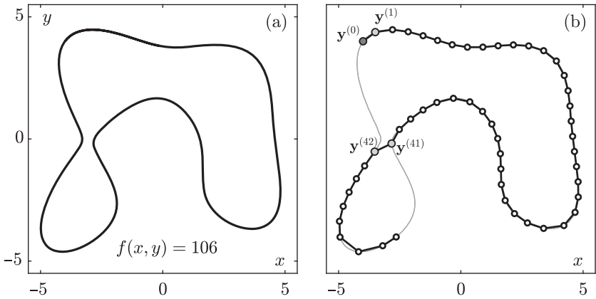
Figure 6.6 Level curve f(x, y) = 106 of Himmelblau's function (6.46). (a) Starting the secant continuation from points \mathbf{y}^{(0,1)} given in (6.47) and (6.48). (b) Failure of the continuation when starting from points (6.49) and (6.50). The correct contour is the underlying gray solid curve.
