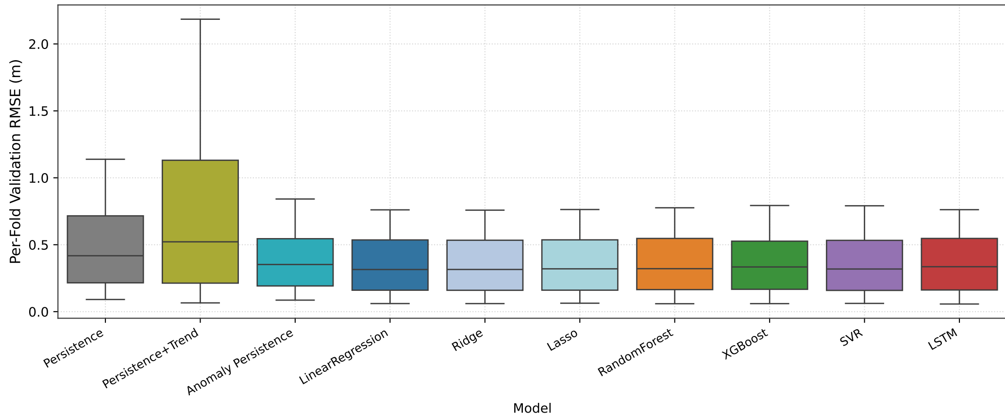
Cross-Validation RMSE Stability Across 12 LOYO Fold Years
