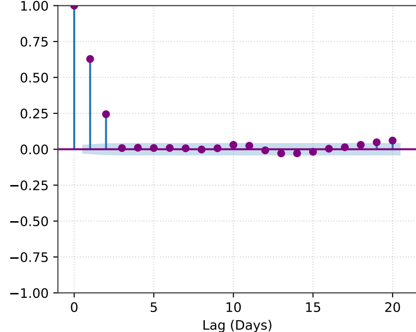
Residual Autocorrelation (ACF)
