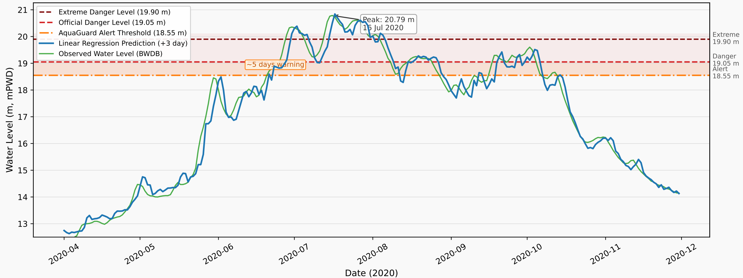
Figure D: AquaGuard Warning Threshold Hydrograph — 2020 Flood Season Bahadurabad Transit Station (SW46.9L), Jamuna River, +3-Day Forecast
