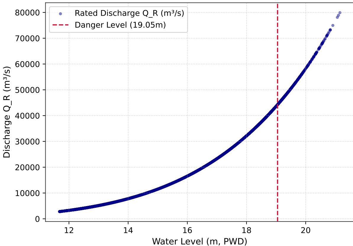
Rating Curve Relationship: Water Level vs Discharge (Bahadurabad)
