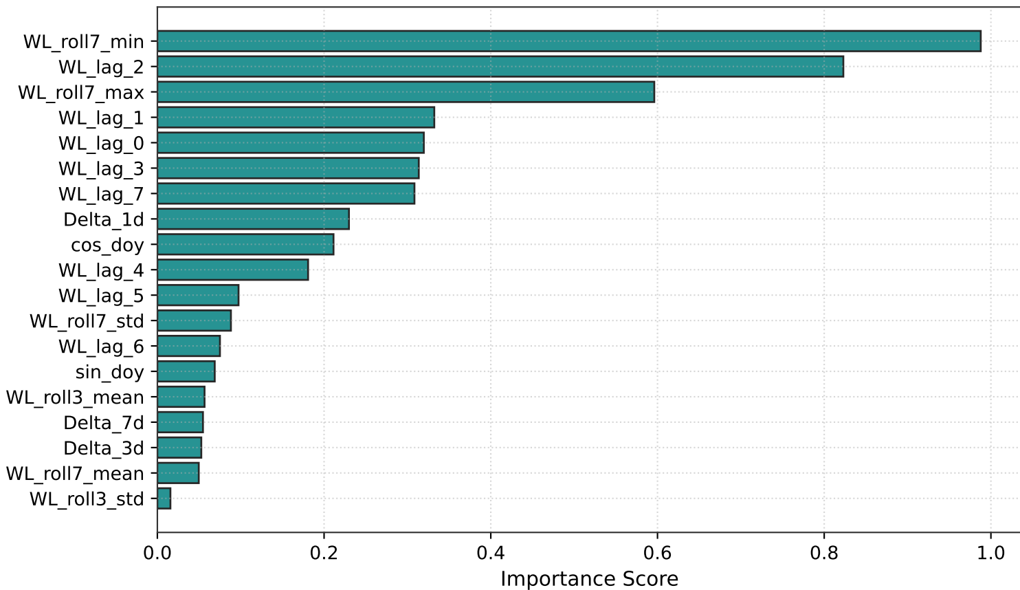
Feature Importance Matrix (Winning Model)
