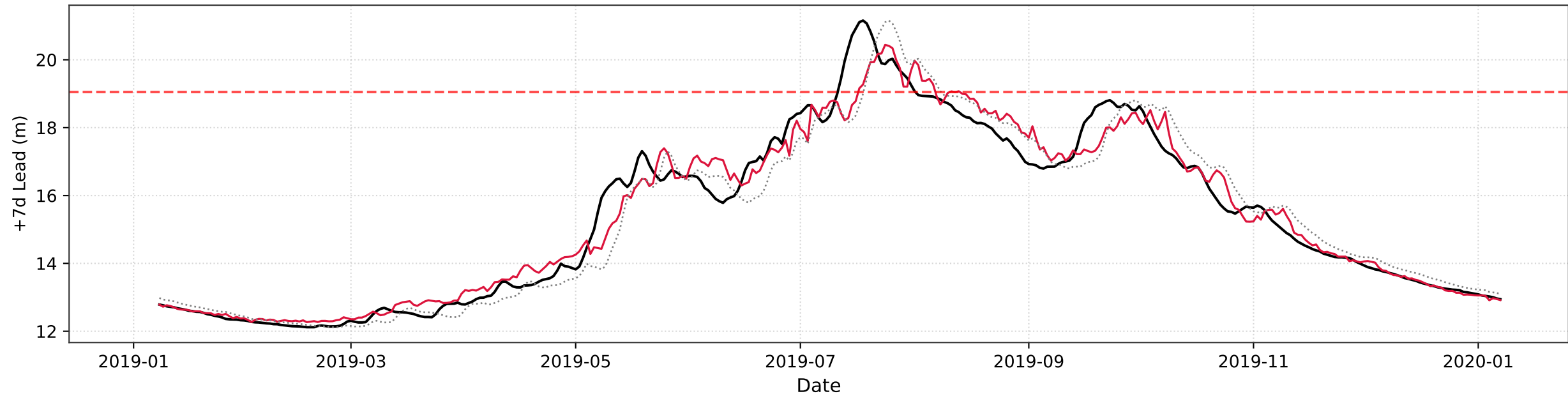
Forecast vs Observed Hydrograph at +7 Day Lead Time
