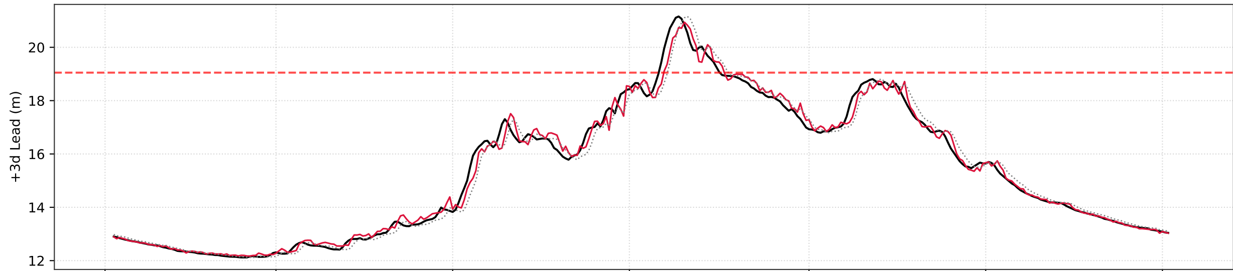
Forecast vs Observed Hydrograph at +3 Day Lead Time
