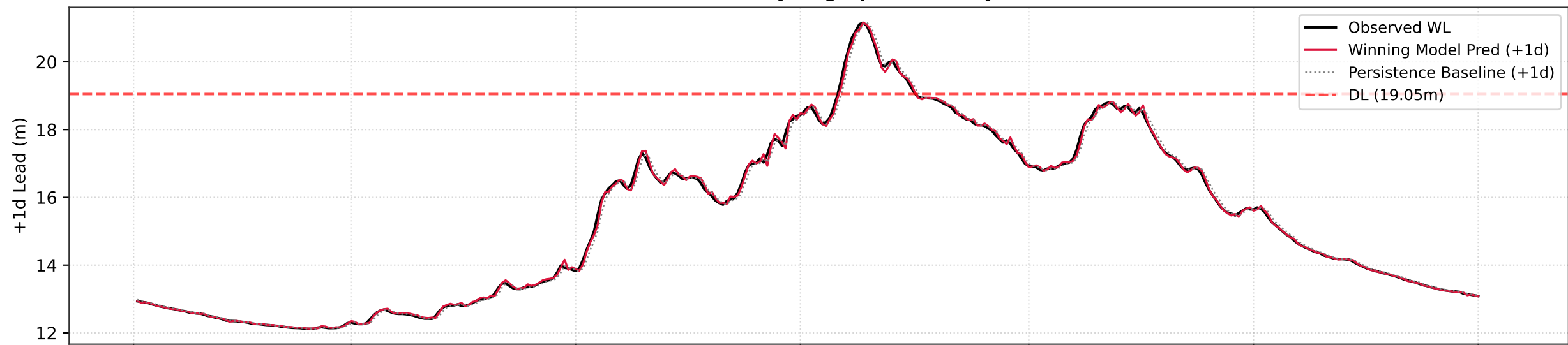
Forecast vs Observed Hydrograph at +1 Day Lead Time
