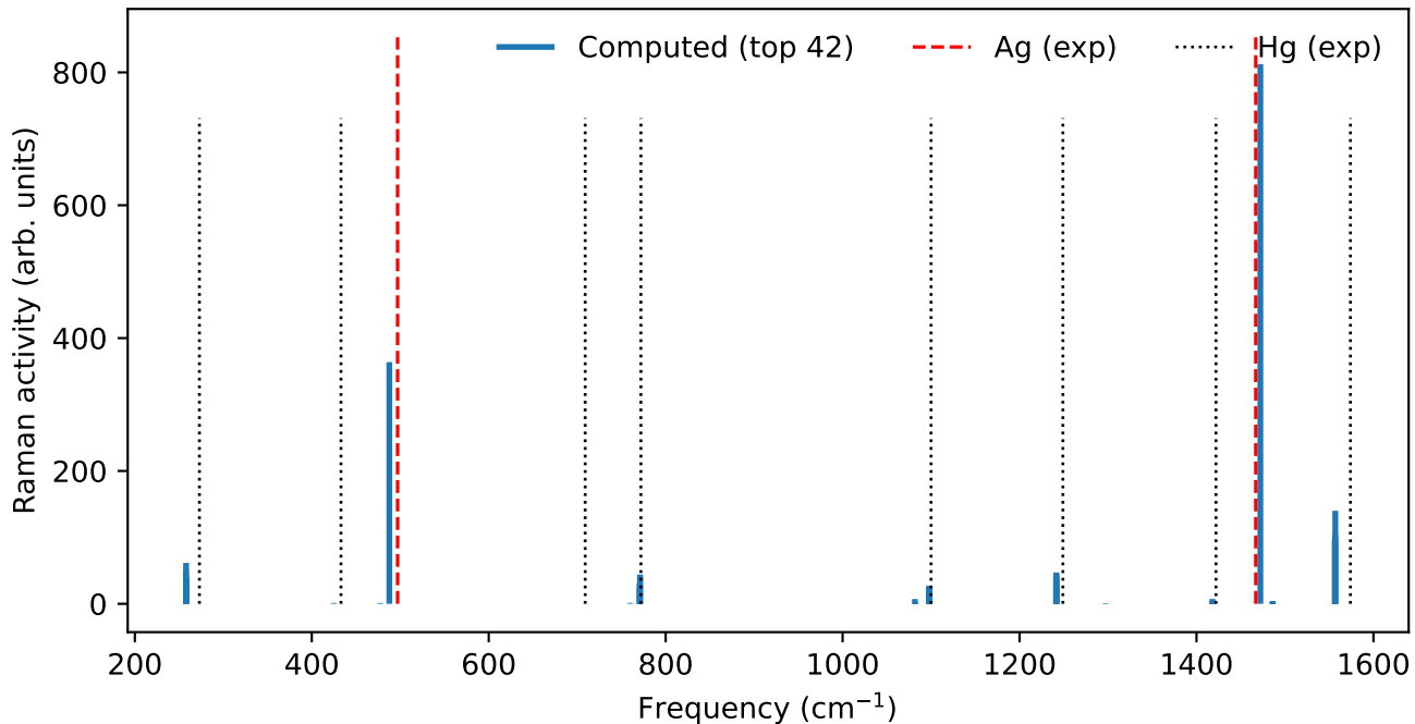
C 60 Raman spectrum — top 42 modes (L = 14 Å, E = 0.05)
