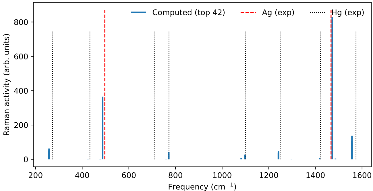
C 60 Raman spectrum — top 42 modes (L = 14 Å, E = 0.10)
