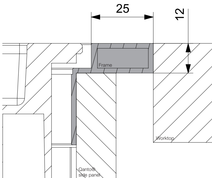
Cross-section frame
