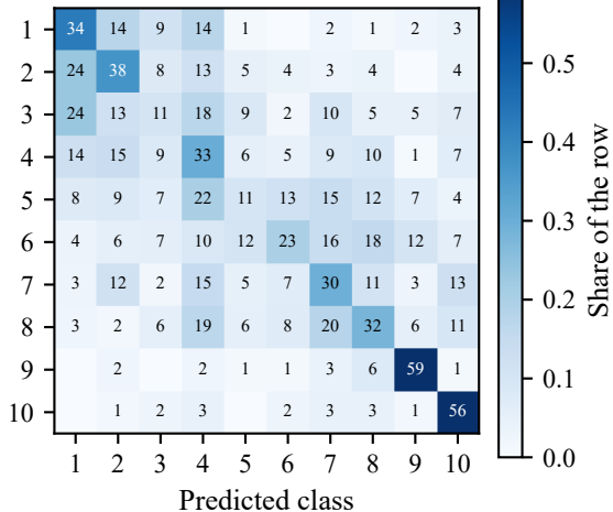
(b) RMEP, fine-tuned
