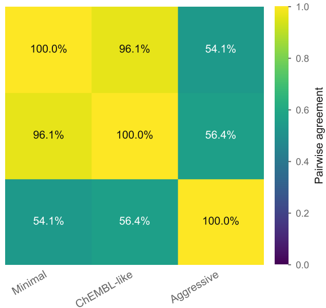
Canonical-SMILES identity
