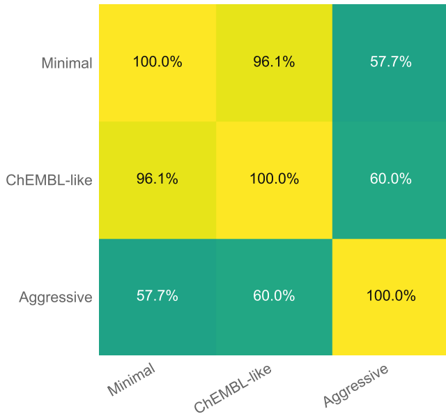
InChIKey identity
