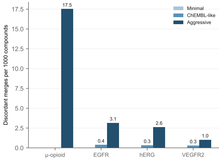
Training labels corrupted by merging
