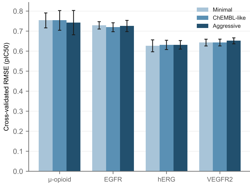
Model performance is unaffected
