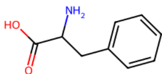
phenylalanine
