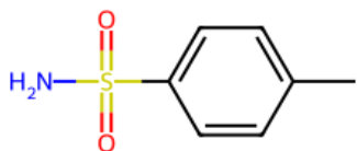
toluenesulfonamide
