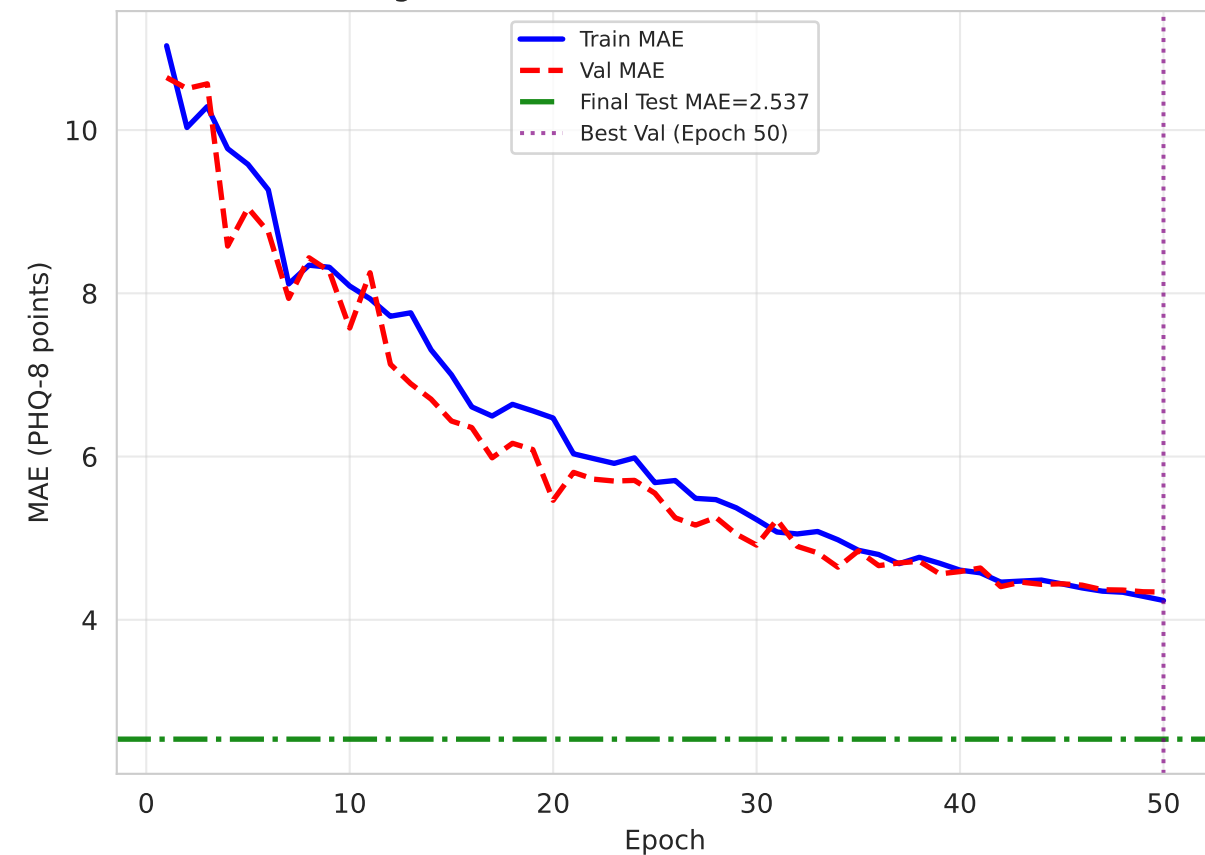
Regression: Mean Absolute Error (MAE)
