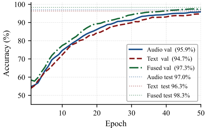
(b) Validation Accuracy
